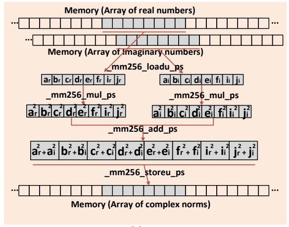
FIGURE 2: Complex norm AVX algorithm using a) Array of Structures (AoS), b) Structure of Arrays (SoA).
