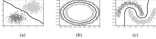
Fig. 2. Figure illustrating boundaries obtained by MSF-watershed. (a) Two blobs dataset (b) Two circles dataset (c) Two moons dataset. All datasets are generated using sklearn [17]. The boundaries are sketched using the 1-Nearest Neighbor classifier as discussed in the text.
