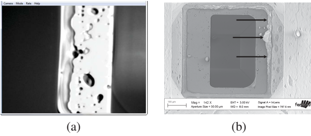
Fig. 7. (a) Image taken by the camera showing the damaged state of the membrane and (b) SEM image showing the contamination at the normally closed port.
