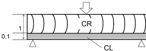
Fig.1: Structure of composite beam
