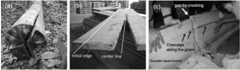
Fig. 1 Distortions due to release of elastic component of the GS in the green wood.
