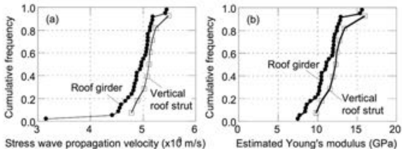
Fig.3: Distribution of Stress wave propagation velocity of frame member and estimated Young's modulus
