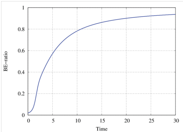
Figure 7. The evolution of the BE ratio starting in the E-regime. Initial conditions are [X_1] = [X_2] = [Y_1] = 1 , [Y_2] = 0 , k_E = k_B = 1 , \phi = 10 , and [X_3] = 50 .
