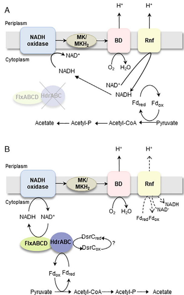
Fig. 4. The central role of HdrA in the pyruvate-based O_2 respiratory growth for ES5 (A) and ESE (B) strains. BD: BD quinol oxidase, Rnf: ferredoxin:NADH oxidoreductase complex, MK/MKH2: menaquinol pool, HdrABC: heterodisulfide reductase complex, FlxABCD: flavin oxidoreductase, Fd red/ox : reduced/oxidized ferredoxin, dsrC: dissimilatory sulfite reductase C. Thick arrows correspond to major fluxes and dashed arrows to minor fluxes.
