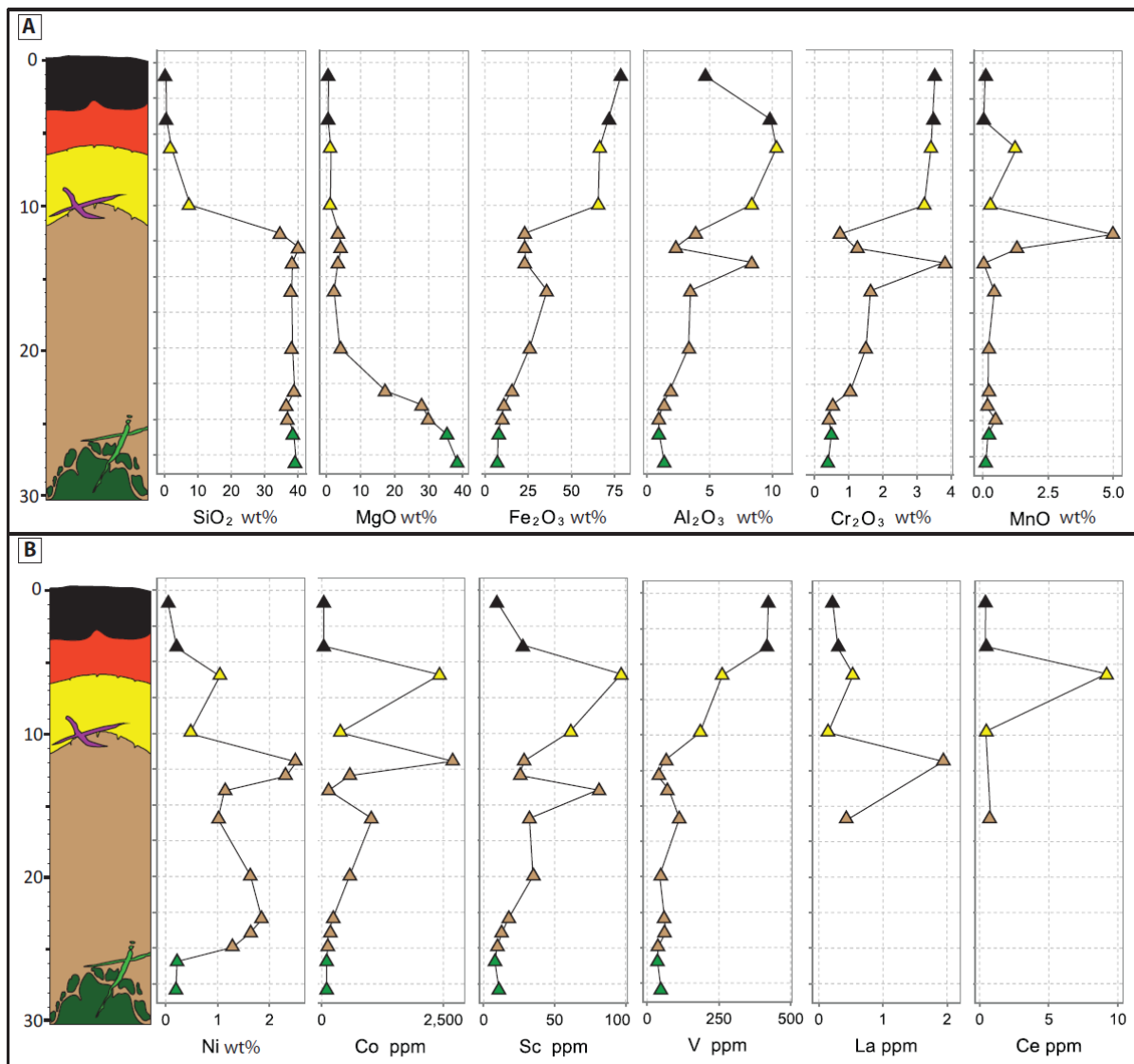
Figure 15: Geochemical evolution along Iherzolite-derived lateritic profile TIEA (Tiébaghi): (A) Major oxides: SiO 2 , MgO, Fe 2 O 3 , Al 2 O 3 , Cr 2 O 3 , MnO (wt%), (B) Economic elements: Ni (wt%), Co (ppm), Sc (ppm), trace and LREE: V, La, Ce (ppm).
