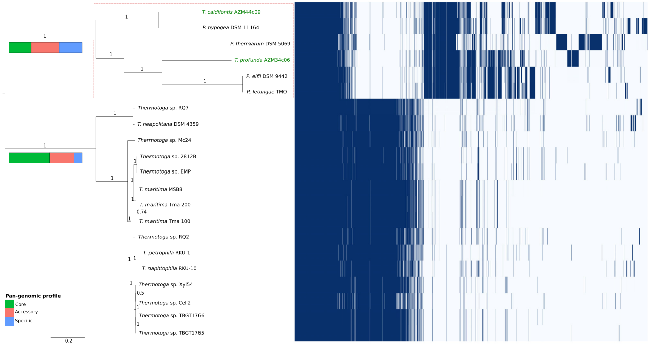
Fig. 3. Core-genome-based phylogeny of the Thermotogaceae family.
