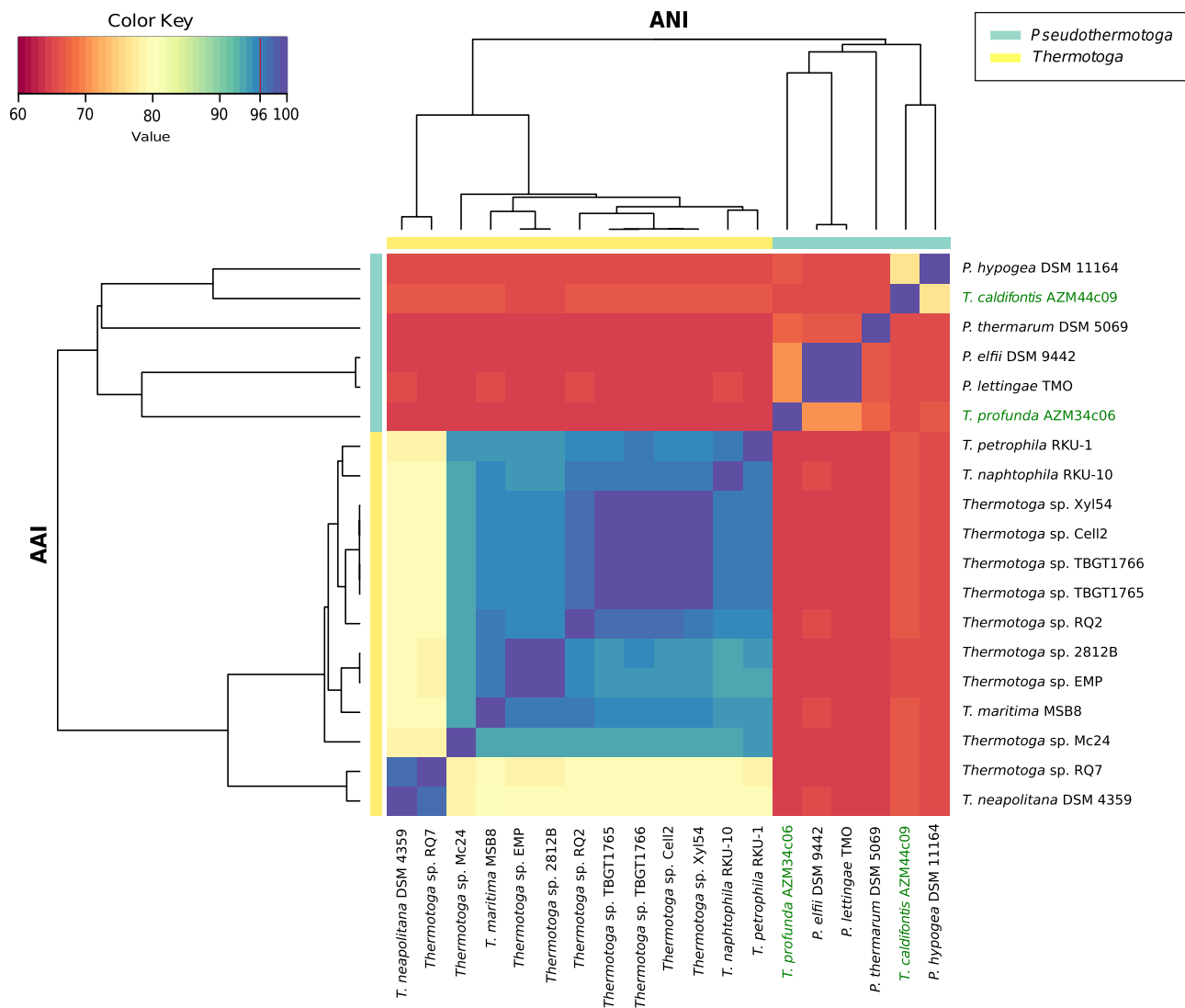
Fig. 5. Whole-genome relatedness within the Thermotogaceae family.
