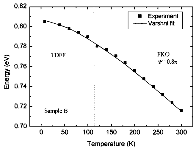
FIG. 5. Temperature dependence of the GaAsSb alloy band gap in sample B (squares extracted from FKO and TDFF theory). Fit to Varshni equation (solid line).
