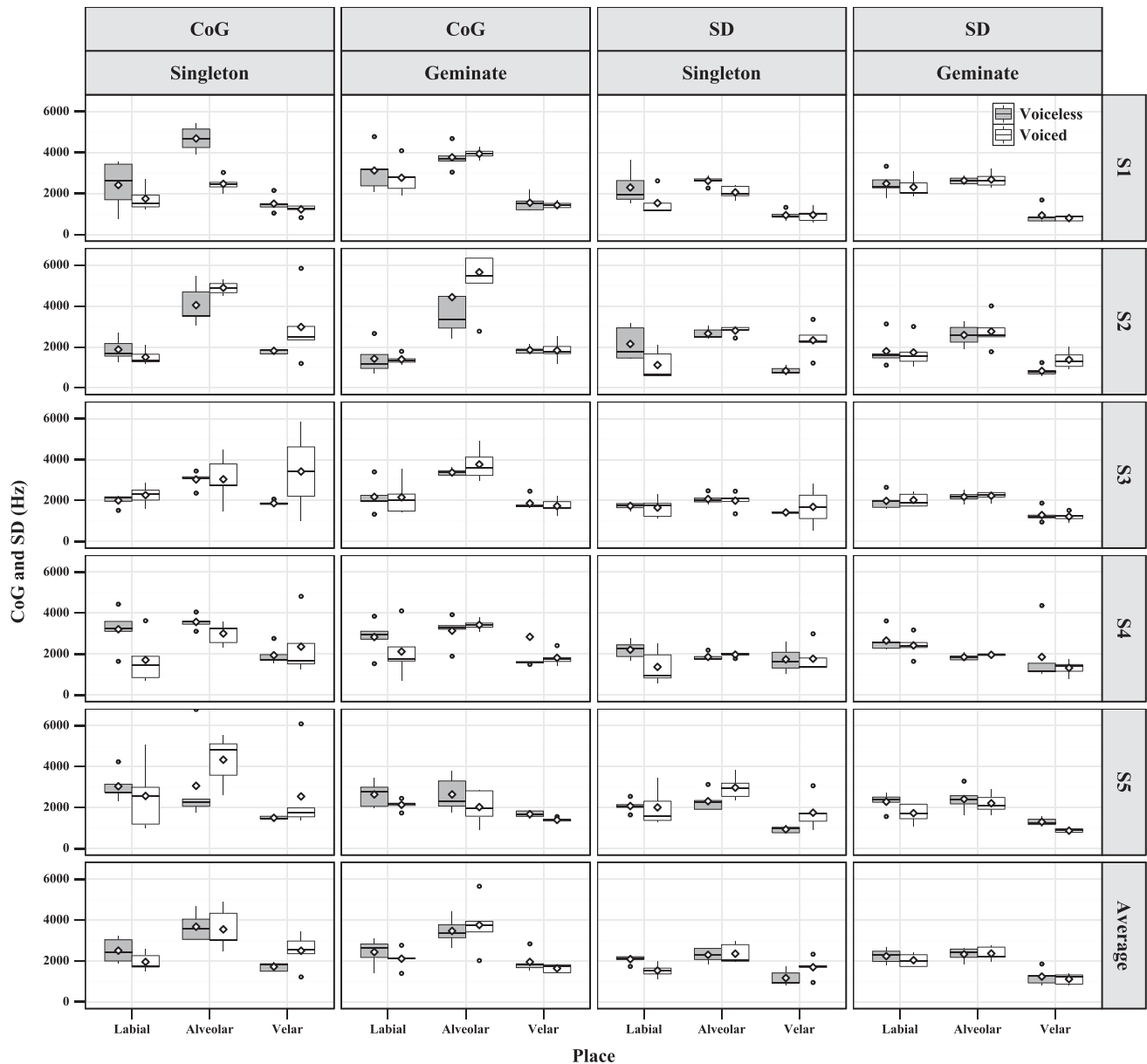
FIG. 7. Boxplots of spectral CoG (left two columns) and spectral SD (right two columns) of C2 stop release bursts in voiceless and voiced singleton and geminate stops of Tokyo Japanese.
