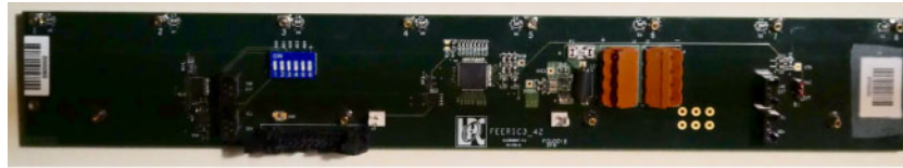
Fig. 78. A front-end board, developed for ALICE, housing the FEERIC ASIC in the center of the board. At the top, the eight pins connecting the readout strips (designed for 4.5 cm readout strips in this case) are visible. The four pins on the bottom of the picture are for grounding. The board shown is 32.5 cm long and 5 cm wide, but the final dimensions will be determined by the optimal BS-CRV segmentation.
