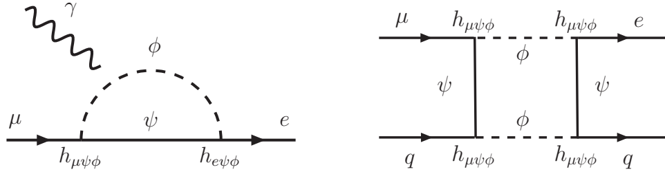
Fig. 5. Schematic representation of photonic contributions to \mu - e flavor transitions (left panel), and of the box-diagram contribution to \mu^- N \rightarrow e^- N conversion (right panel), in the presence of new fermions ( \psi ) and new vector/scalar bosons ( \phi ).
