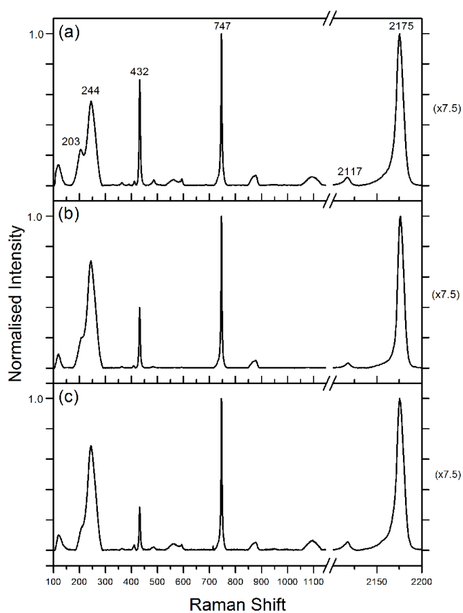
Figure 6. The mean normalised Raman spectra with baseline subtraction for the 2D platelets, 1\ \mu\text{m} and 400\ \text{nm} samples are shown in (a), (b) and (c) respectively. The spectral regions of 100\text{--}1150\text{ cm}^{-1} and 2100\text{--}2200\text{ cm}^{-1} can be seen for all samples, with the main Raman peaks of CuSCN labelled in spectrum (a). The normalised intensity in the 2100\text{--}2200\text{ cm}^{-1} wavenumber region, has been rescaled in order to plot the intense Raman response of the 2175\text{ cm}^{-1} peak on the same scale, the dividing factor of 7.5 was used and hence the right scale indicates the x7.5 factor that has to be used to interpret the higher wavenumber region.
