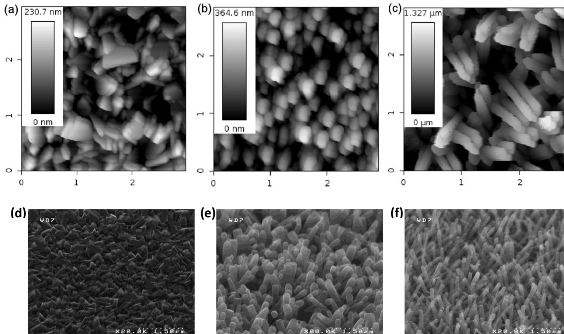
Figure 1. AFM images (a-c) taken with dimensions 3\ \mu\text{m} \times 3\ \mu\text{m} ; the corresponding black-to-white height scales are shown individually on each scan. SEM images (d-f) were taken with \times 20\text{k} magnification. The 2D platelets, 400\ \mu\text{m} and 1.4\ \mu\text{m} samples are shown in AFM images (a), (b) and (c) respectively and in SEM images (d), (e) and (f) respectively.
