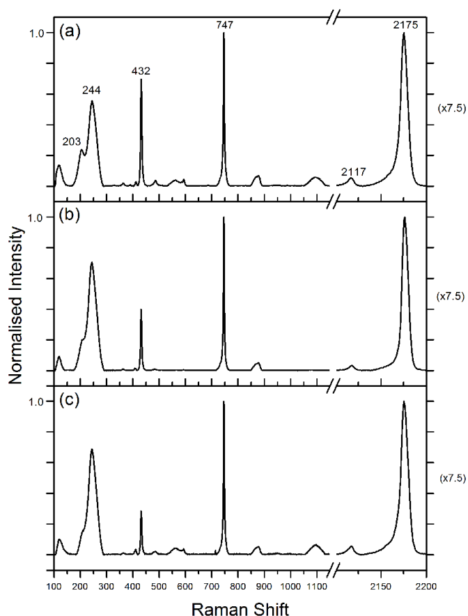
Figure 6. The mean normalised Raman spectra with baseline subtraction for the 2D platelets, 1 \mu\text{m} and 400 nm samples are shown in (a), (b) and (c) respectively. The spectral regions of 100-1150 \text{cm}^{-1} and 2100-2200 \text{cm}^{-1} can be seen for all samples, with the main Raman peaks of CuSCN labelled in spectrum (a). The normalised intensity in the 2100-2200 \text{cm}^{-1} wavenumber region, has been rescaled in order to plot the intense Raman response of the 2175 \text{cm}^{-1} peak on the same scale, the dividing factor of 7.5 was used and hence the right scale indicates the x7.5 factor that has to be used to interpret the higher wavenumber region.
