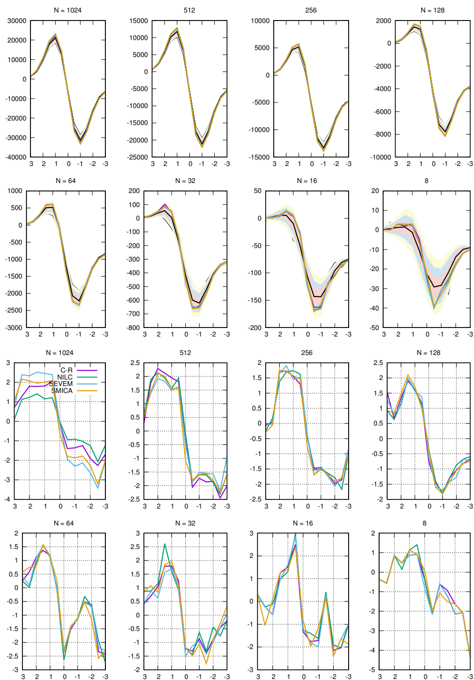
Fig. B.6. EC_{\text{rel}} graphs for resolutions between N = 1024 and N = 8 . Top two rows: observed curves from all the simulation methods, and the expected (black) curve computed from 100 SMICA simulations, along with bands drawn up to 3\sigma . Also plotted underneath are 100 curves from the individual simulations. Bottom two rows: curve presenting the difference between the observations and simulations in terms of the number of standard deviations for the various temperature thresholds.
