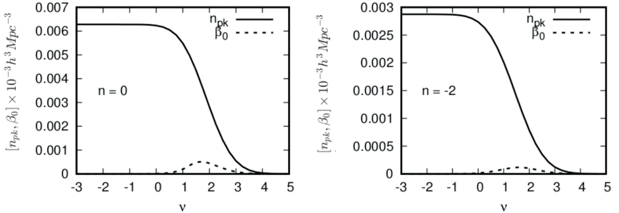
Figure 21. Cumulative number distribution of peaks and the distribution of islands (zeroth Betti number) for comparison as a function of density threshold. The left-hand panel presents the graphs for the n = 0 model, and the right-hand panel plots it for the n = -2 model.
