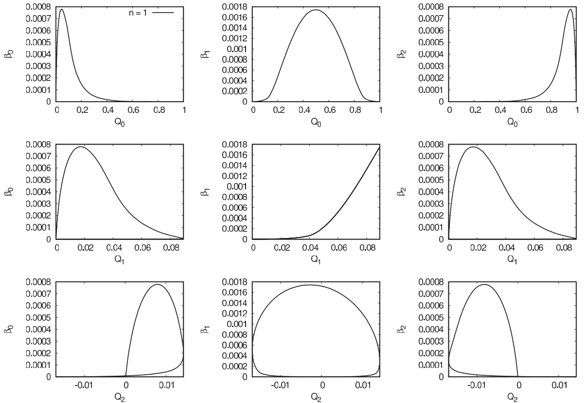
Figure 25. Betti numbers versus the Minkowski functionals.
