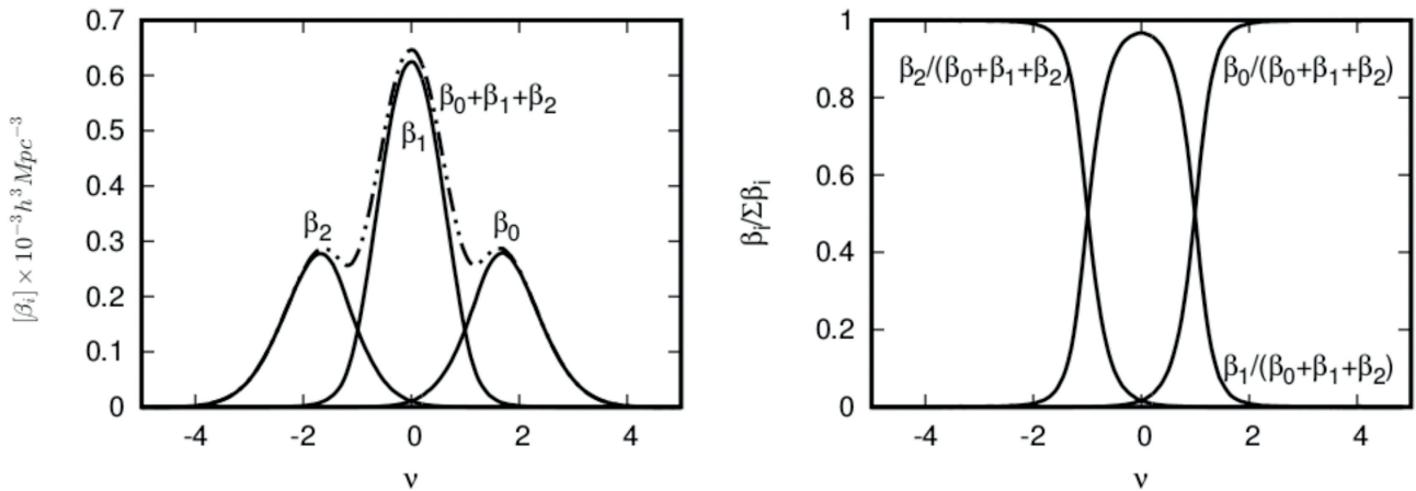
Figure 6. Figure illustrating the dominance of different Betti numbers in the different density threshold regions. The left-hand panel plots the sum of Betti numbers for the different thresholds, along side the individual Betti numbers. The right-hand panel presents the ratio of the individual Betti numbers to their sum as a function of the density threshold.
