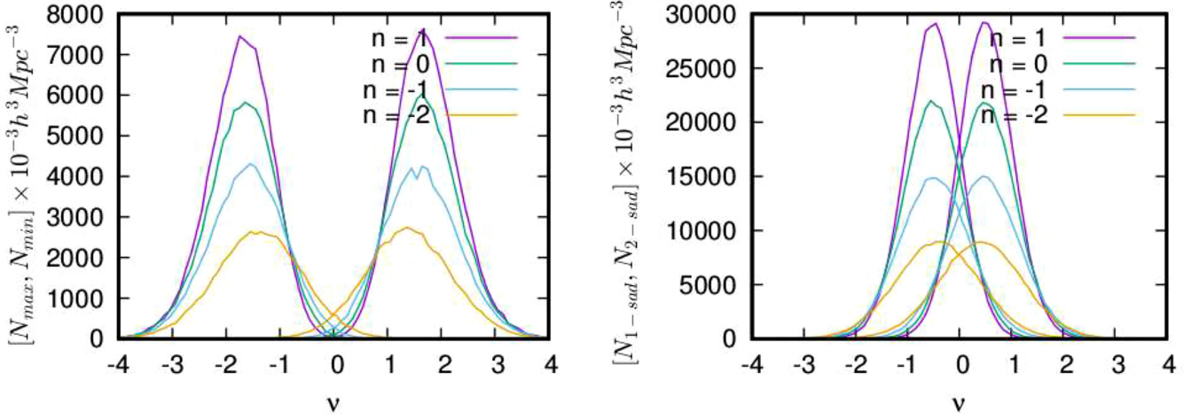
Figure 20. Number distribution of critical points as a function of the spectral index. The left-hand panel plots the distribution of the maxima/minima as a function of the spectral index and density threshold. The right-hand panel plots the same for 1- and 2-saddles.
