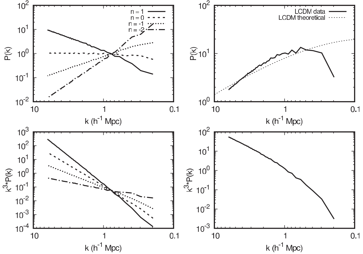
Figure 4. The power spectrum P(k) , as well as power spectrum per unit logarithmic bin k^3 P(k) . Graphs are presented for the different spectral indices of the power-law model (left-hand column), as well as the LCDM model (right-hand column). The power-law spectra are scaled such that different models have the same variance of the density fluctuations, when filtered with a top hat filter of radius 8 h^{-1} Mpc.
