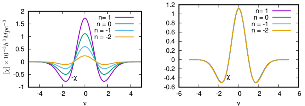
Figure 15. Scaling behaviour of the Euler characteristic curves for the power-law models. Left-hand panel: unscaled Euler characteristic curves for the power-law models. Right-hand panel: scaled curves for the same. The curves for the different models are scaled so that their amplitudes coincide. The scaled curves are indistinguishable from each other.
