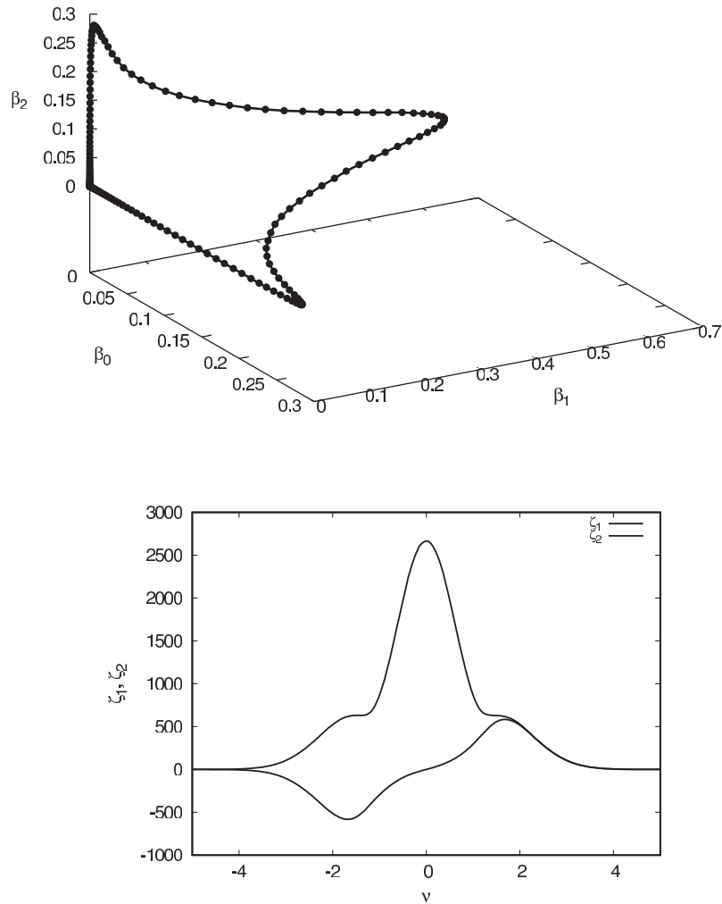
Figure 16. \beta -track (top) and \zeta -track (bottom) for a typical Gaussian field model. They represent orthogonal information to the Euler characteristic, see the text for details.
