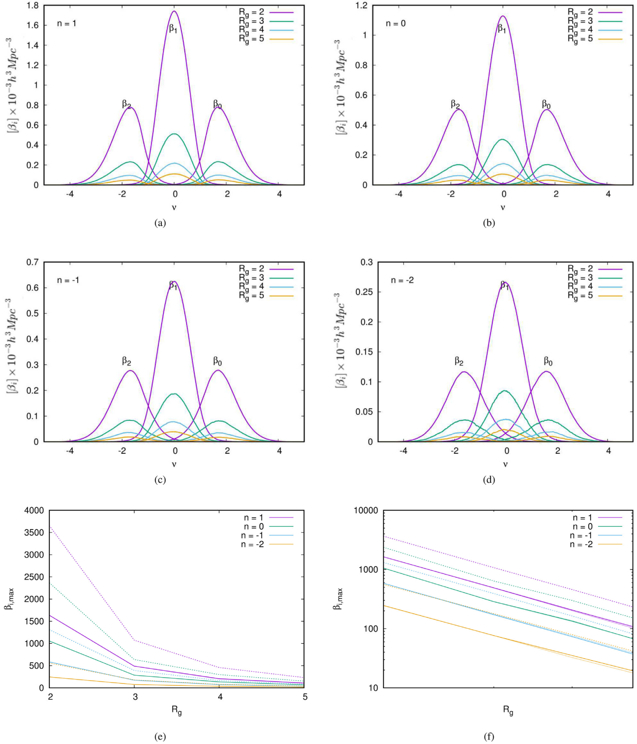
Figure 12. Dependence of the amplitude of Betti number curves on the filter radius R_g . Panels (a) to (d): Betti number curves for the n = 1, 0, -1, and -2, respectively, where for each model, the field is smoothed by a Gaussian kernel of varying radii R_g = 2, 3, 4, and 5. Panel (e): Graph presenting the amplitude of the Betti curves as a function of smoothing radius. Curves with the same colours represent the same model. The dotted curves are for \beta_1, while the solid and the dashed curves represent \beta_0 and \beta_2, respectively. Panel (f): Same as panel (e), but on a logarithmic scale.
