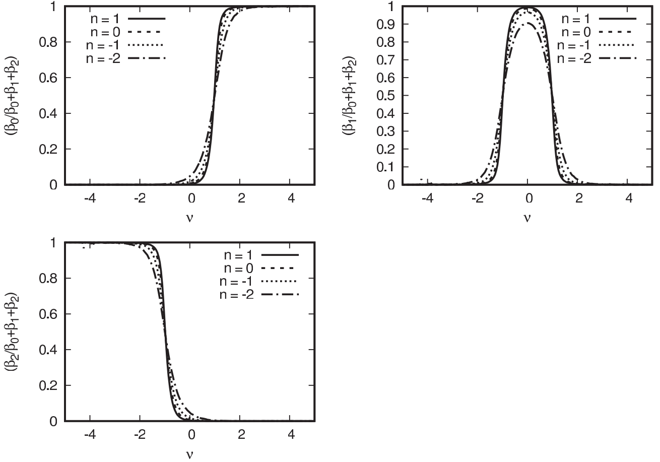
Figure 10. The fractional contribution of islands, tunnels, and voids to the sum of Betti numbers in all three dimensions for rms threshold range between (-5\sigma; 5\sigma) for the different power-law models. Top-left: \beta_0/(\beta_0 + \beta_1 + \beta_2) – fractional contribution of islands to the total sum of Betti numbers. Top-right: \beta_1/(\beta_0 + \beta_1 + \beta_2) – fractional contribution of tunnels to the total sum of Betti numbers. Bottom-left: \beta_2/(\beta_0 + \beta_1 + \beta_2) – fractional contribution of voids to the total sum of Betti numbers.
