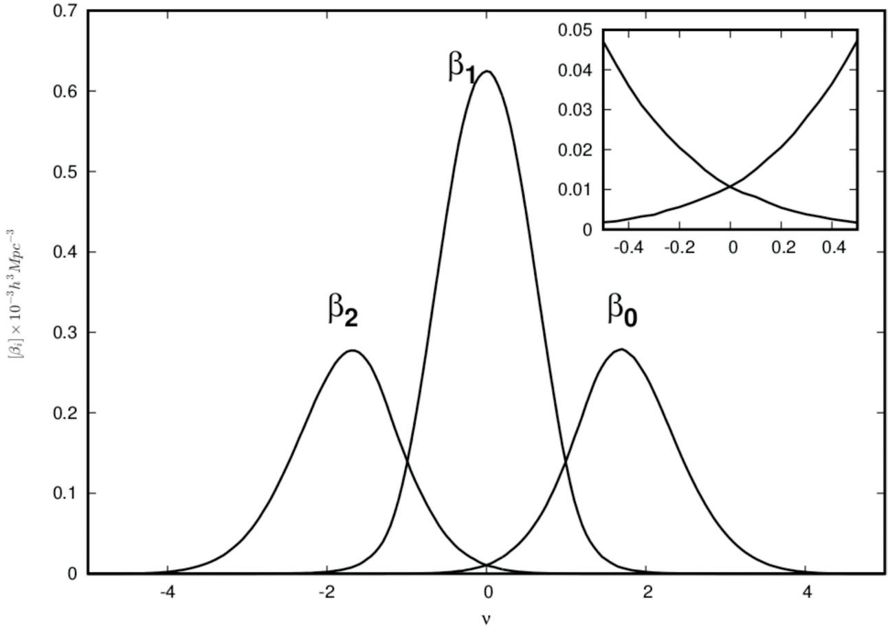
Figure 5. The Betti numbers for the n = -1 model. It is evident that the different Betti numbers dominate the topology in the different density thresholds regions, and also the Euler characteristic curve. For high thresholds, \beta_0 is the dominant topological feature. For intermediate thresholds, \beta_1 dominates, while for low thresholds \beta_2 is the dominant topological entity. Inset: The zone of overlap between \beta_0 and \beta_2 curves, at the median density threshold. Both the quantities are non-unity, indicating that the manifold is not a single connected surface, and hence does not exhibit pure Sponge-like topology.
