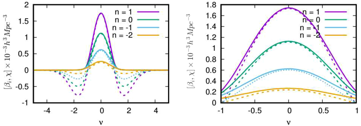
Figure 14. Comparison of relative contributions of \beta_1 versus Euler characteristic. As the spectral index lowers, the peak of the Euler characteristic has progressively lower amplitude compared to the \beta_1 curve.
