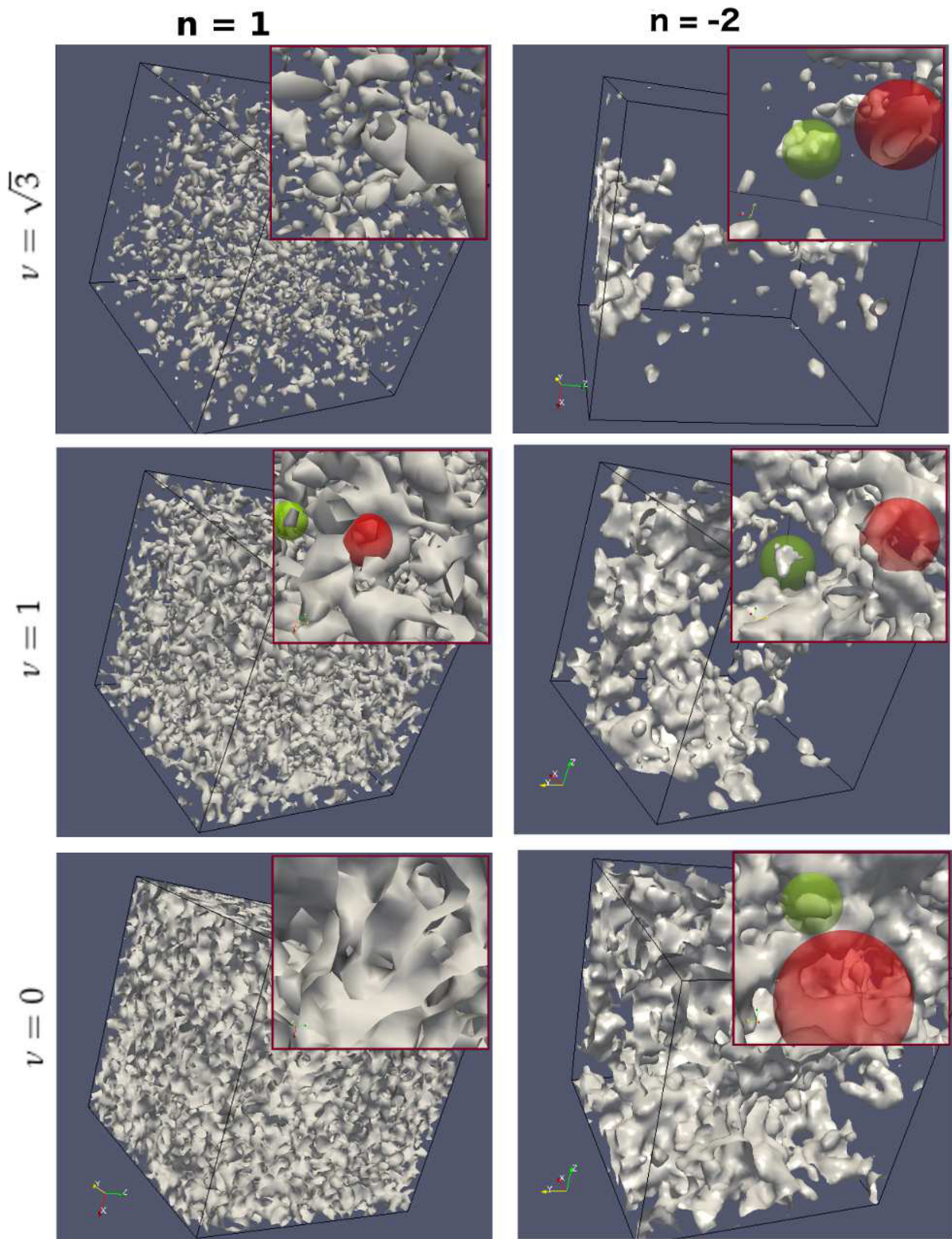
Figure 1. Isodensity surfaces denoting the structure of the field for three different density thresholds v = \sqrt{3} , 1, and 0, for the n = 1 and the n = -2 models. The left-hand column presents the isodensity surfaces for the n = 1 model and the right-hand column presents the contour surfaces for the n = -2 model. Examples of typical tunnels are enclosed in translucent red spheres; examples of typical isolated islands are enclosed in green spheres. The topology of the contour surfaces shows a dependence on the choice of the power spectrum, as well as the density threshold.
