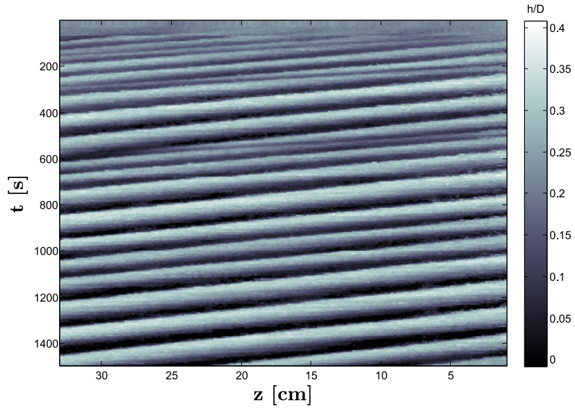
FIGURE 5. Space-Time diagram for \Phi = 0.05 - \theta = 0.074 - U_0 = 0.11 \text{ m/s} - Re_0 = 2937 .
