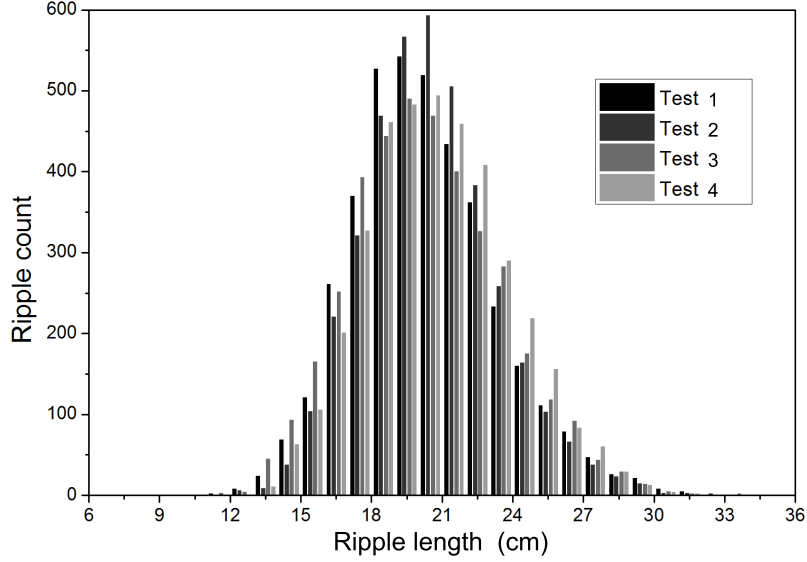
FIGURE 12. Distribution of the length of saturated ripples for \Phi = 0.05 - \theta \approx 0.13 - U_0 \approx 0.13 m/s - Re_0 \approx 3500 .
