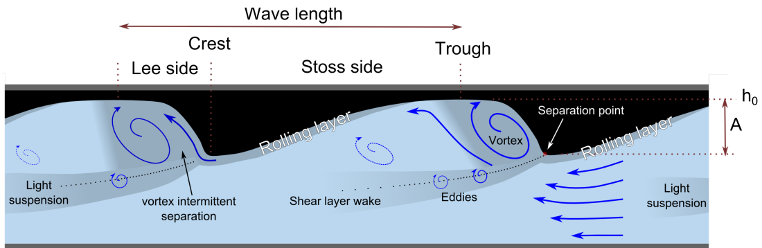
FIGURE 7. Explanatory diagram of fluid and solid flow behaviour in the case of vortex ripples.
