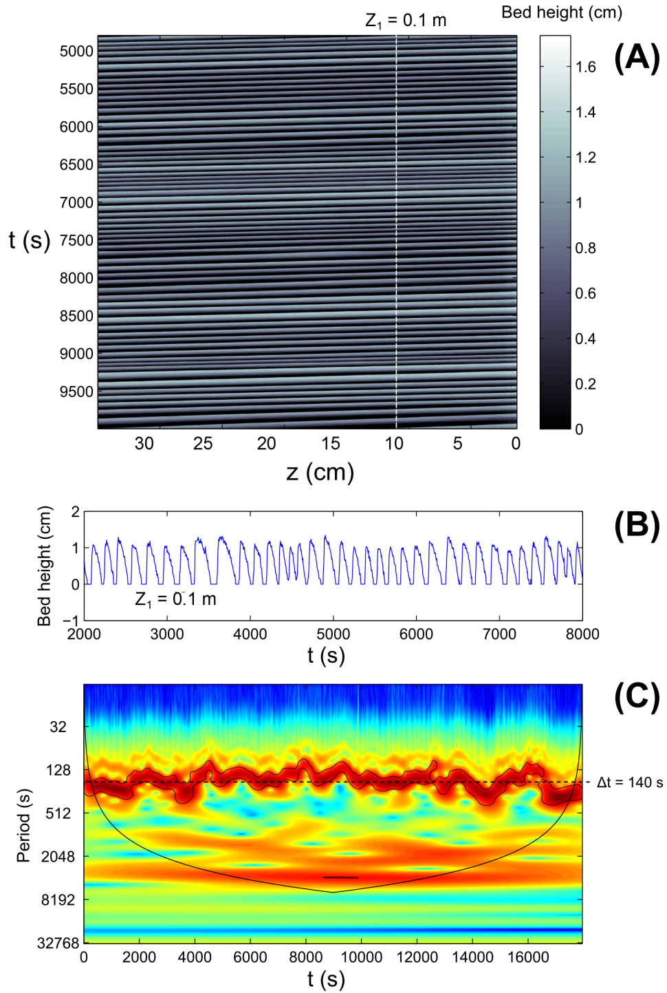
FIGURE 9. (A) Space-Time diagram, (B) Bed height versus time for a specific spatial position ( z_1 = 0.1 m), (C) Result of the wavelet analysis, for \Phi = 0.05 - \theta = 0.063 - U_0 = 0.10 m/s - Re_0 = 2814 .
