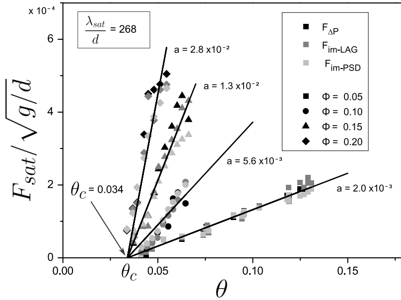
FIGURE 14. Dimensionless frequency of saturated ripples as a function of \theta and \Phi .
