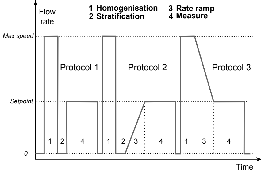
FIGURE 10. Illustration of protocols used to check the unicity of the saturated state.
