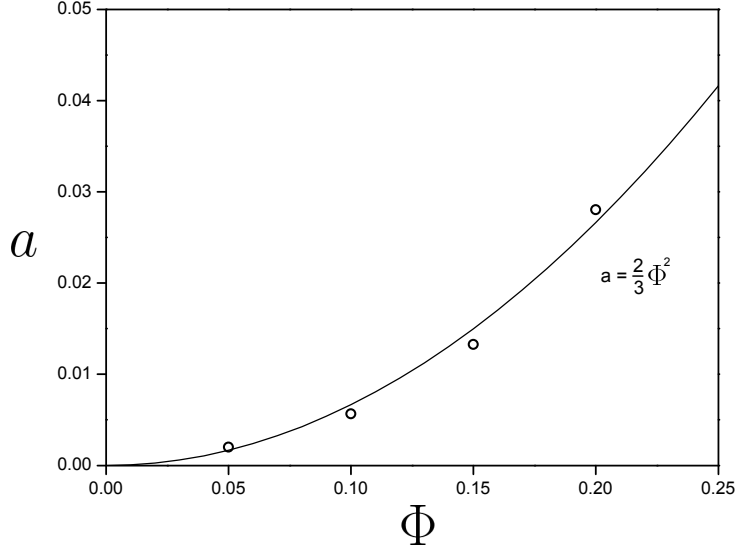
FIGURE 16. Evolution of a versus \Phi .
