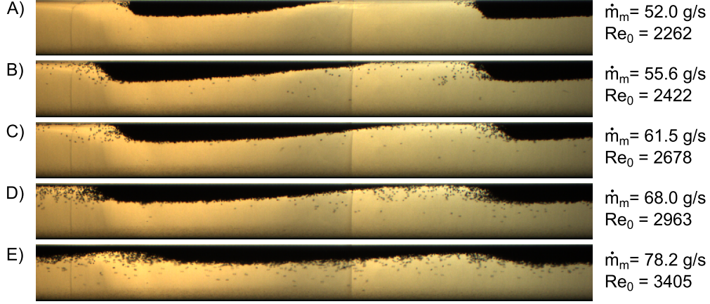
FIGURE 3. Photographs of saturated ripples for \Phi = 0.05 , illustrating the gradual extinction of bedforms with an increase in the flow rate
