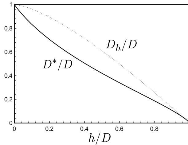
FIGURE 17. Evolution of D^*/D and D_h/D depending on h/D according to Peysson et al. (2009)
