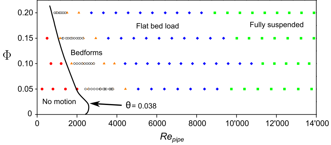
FIGURE 4. Map of the flow patterns observed with a mixture of water and 756 \mu\text{m} polypropylene particles in a horizontal pipe of 3 cm diameter ; (o) are the measurements used in this study; (-) is the 0.038 iso-Shields number predicted by the model proposed by Peysson et al. (2009)
