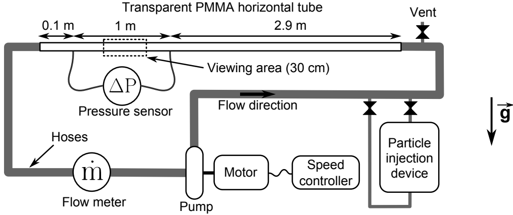
FIGURE 1. Schematic of the experimental set-up
