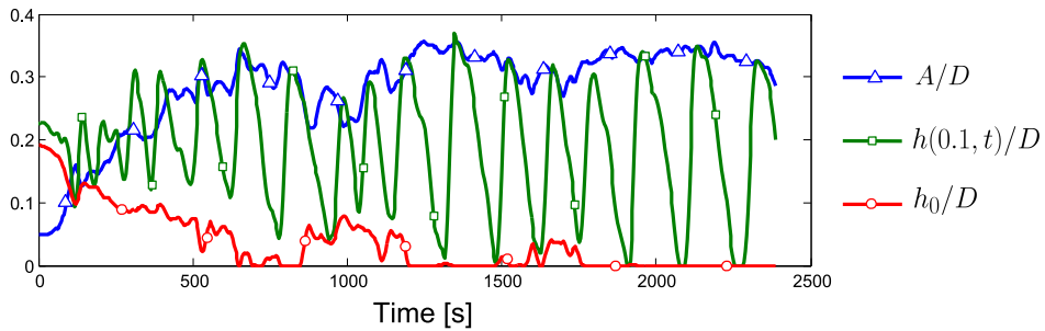
FIGURE 6. A/D, h_0/D, h(0.1, t)/D versus time for \Phi = 0.05 - \theta = 0.074 - U_0 = 0.11 \text{ m/s} - Re_0 = 2937 .
