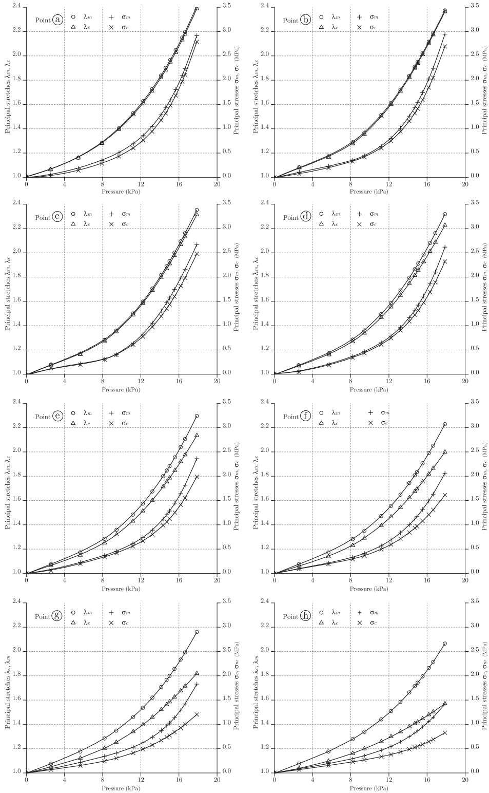
Fig. 3. Bulge test deformation history for points a to h. Principal stretches ( \lambda_m, \lambda_c ) and Cauchy principal stresses ( \sigma_m, \sigma_c ) are presented respectively on left and right axis according to the inflating pressure ( p ).
