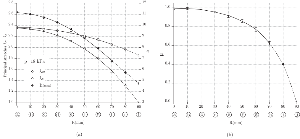
Fig. 4. (a) Highest deformation level experienced on the first biaxial tensile load ( p = 18 kPa) for each meridional point (a to j) in terms of principal stretches ( \lambda_m, \lambda_c ) and first invariant ( I_1 ); (b) Mean value and range of biaxiality ratio ( \mu ) during all pressure load steps. Points i and j were extrapolated using a polynomial approximation (dotted lines).
