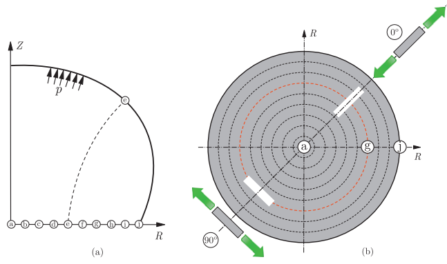
Fig. 2. Schematic representation of biaxial preconditioning method and principal stretches: (a) axisymmetric representation of the bulge test with the interest points; (b) Illustration of the cut subsamples over different directions in the circular membrane.
