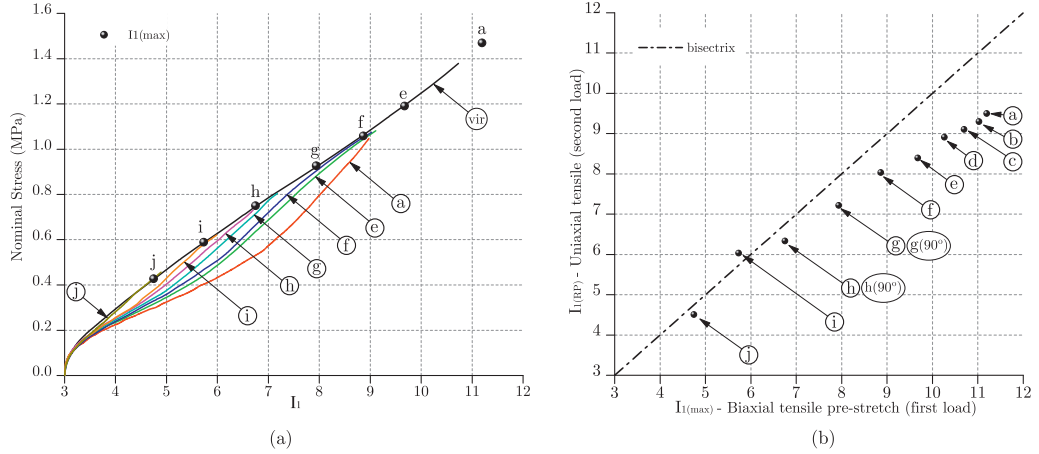
Fig. 9. Influence of the first biaxial tensile loading on uniaxial tensile test response. (a) Uniaxial tension performed at 0^\circ with respect to the meridional direction for points (a, e, f, g, h, i, and j – represented by solid lines) and the maximal first invariant I_{1(\max)} (dots) reached during the biaxial first load (from Fig. 4(a)). (b) Relation between the maximal first invariant I_{1(\max)} and the value of I_{1(RP)} when the second load curve comes back on the reference first loading curve (vir-curve).
