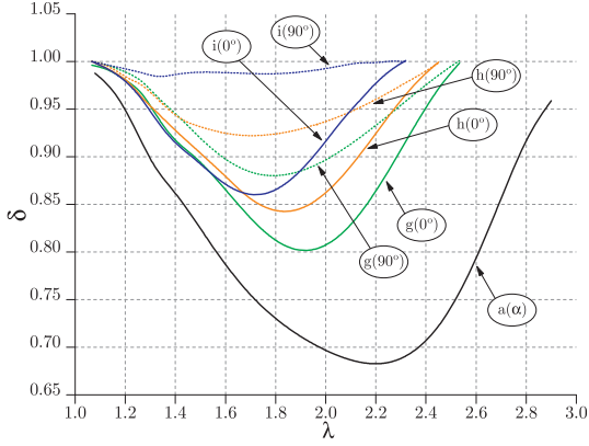
Fig. 8. Stress ratio between the virgin uniaxial tensile load curve ( vir ) and the second load for the uniaxial extension, performed on meridional ( 0^\circ ) and circumferential ( 90^\circ ) specimens, for points a , g , h , and i .
