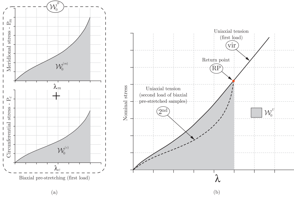
Fig. 11. First and second load strain energy schema. (a) The strain energy decomposition for the biaxial pre-stretching. (b) The equivalent energy ( \mathcal{W}_0^D ) evaluated until the return point (RP) of a given biaxial pre-stretched sample on the uniaxial first load reference curve (vir).
