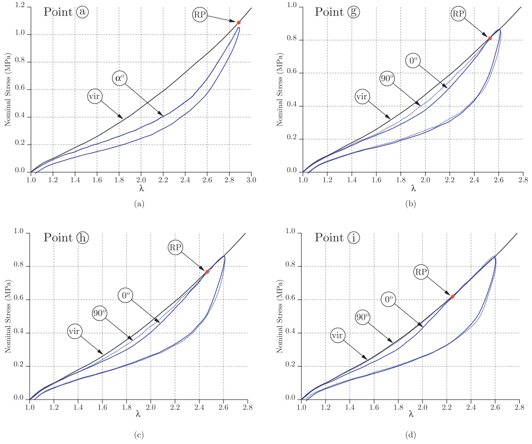
Fig. 6. Second uniaxial tensile load (and unload) curves of specimens a , g , h and i cut from the bulge plate at 0^\circ and 90^\circ with respect to the meridional direction. Note that, for point a , only one curve is presented since the all directions are equivalent.
