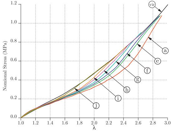
Fig. 5. Influence of the first biaxial tensile load on second uniaxial tensile test response. Uniaxial tension performed in the meridional direction ( 0^\circ ) for the subsamples a, e, f, g, h, i, and j.
