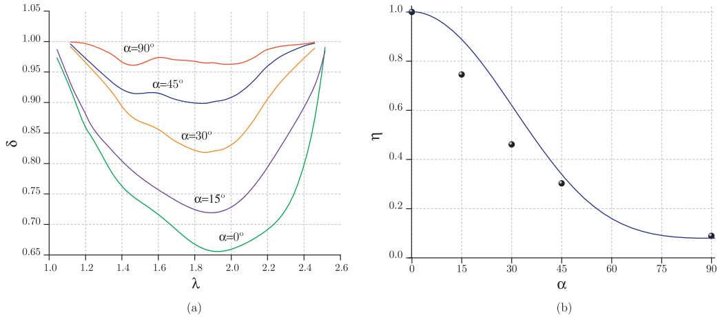
Fig. 7. (a) Stress ratio between the virgin uniaxial tensile load curve and the set of subsamples orientated at 0^\circ , 30^\circ , 45^\circ and 90^\circ (perpendicular) directions. (b) Ratio of energy loss according to the different loading angles.
