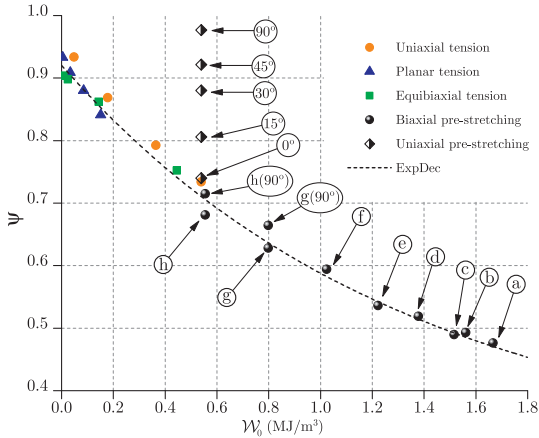
Fig. 10. Strain energy ratio ( \psi ) between second loading (uniaxial tension) and different tensile first loadings. Points are fitted by an exponential decay function.
