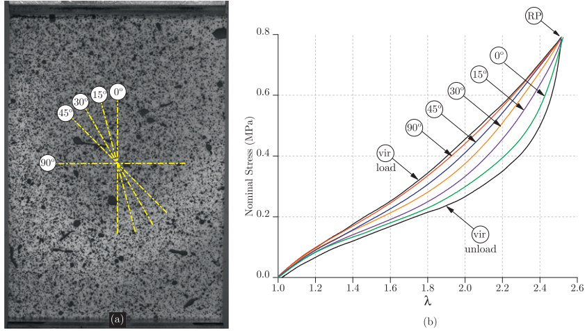
Fig. 1. (a) Preconditioned large sample with the representation of different orientations of the tensile test cut specimens. (b) Induced anisotropy represented by the superposed uniaxial stress–strain responses for the different angles between the first and second loading directions. Curves are compared with the uniaxial tensile curve (load-unload) of a virgin specimen.
