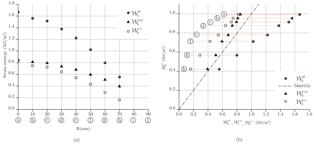
Fig. 12. Bulge test strain energy analysis.
