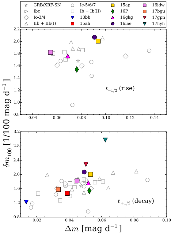
Figure 13. (Top) \delta m_{100} as a function of t_{-1/2} in units of \text{mag d}^{-1} . (Bottom) \delta m_{100} as a function of t_{+1/2} in units of \text{mag d}^{-1} .
