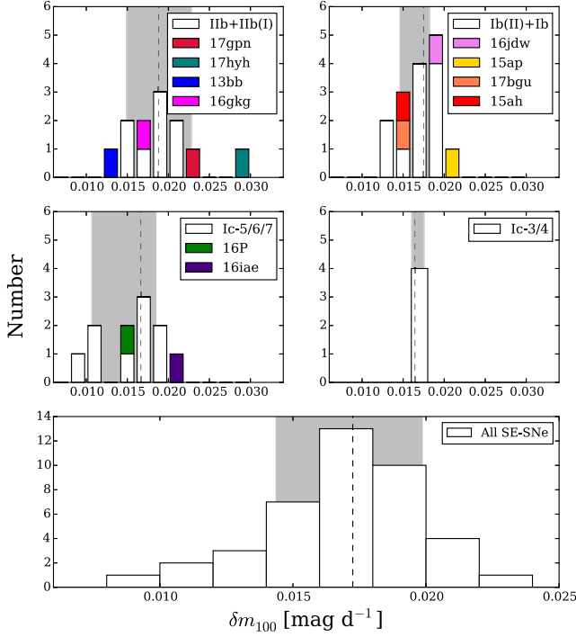
Figure 12. (top) The distribution of late time decay rates for SE-SNe; the median is \sim 0.017 \text{ mag d}^{-1} for all SN types. Only SN 2013bb has had host-galaxy flux subtracted, but the effect of this on \delta m_{100} was found to be negligible at this phase, \sim 0.001 \text{ mag d}^{-1} . The dashed line and grey regions are as in Fig. 9.
