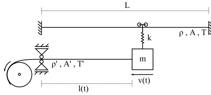
Figure 1 – The complete mechanical system
