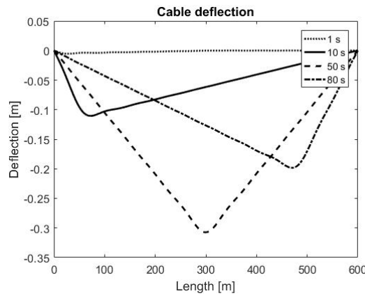
Figure 2 – Deflection of the cable with a moving load
