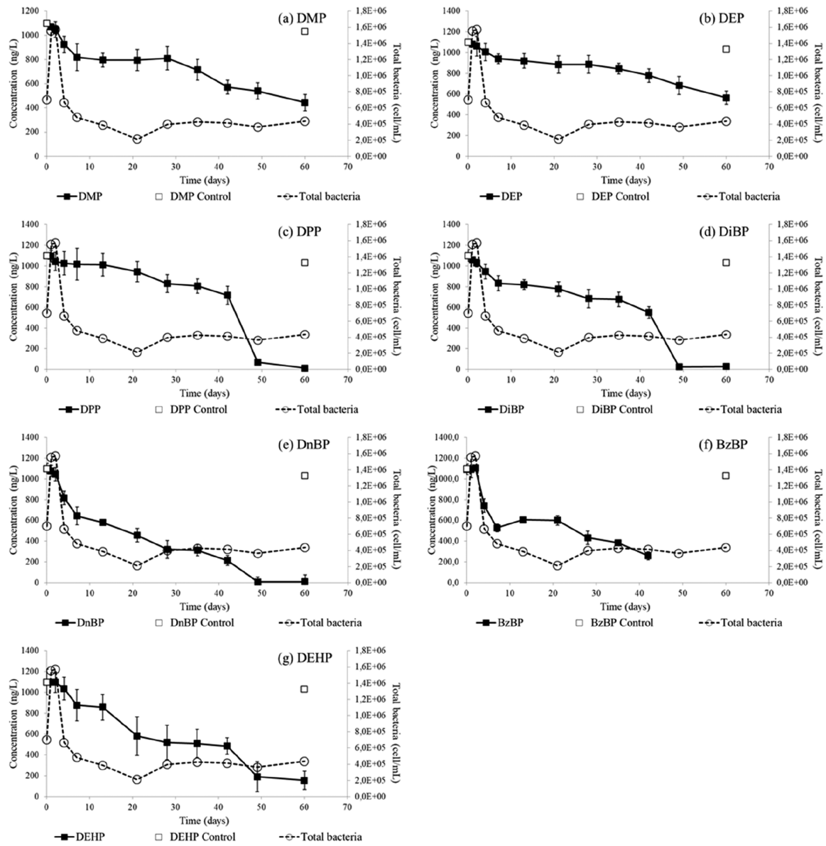
Figure 4. Bacterial degradation of the 7 PAEs in seawater at 22 °C and in the dark condition. (a) DMP, (b) DEP, (c) DPP, (d) DiBP, (e) DnBP, (f) BzBP, and (g) DEHP kinetics of degradation. Abiotic samples poisoned with sulfuric acid were used as controls in this study at t_0 and t_{\text{final}} . Total bacteria include LNA and HNA cell abundance.
