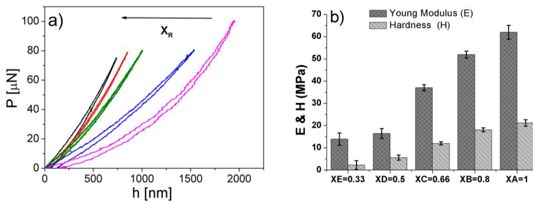
Figure 2: Mechanical properties of castor oil hybrid nanofilms measured by nano-indentation: (a) Loading force ( P ) as a function of depth by varying X_R ratio and (b) the extracted Young's modulus and hardness for each X_R ratio. The maximum load for X_A - X_D was 80 \mu\text{N} and for X_E 100 \mu\text{N} .
