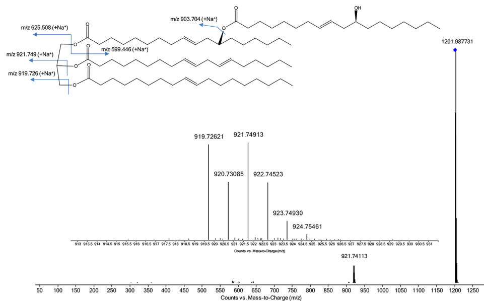
Figure 2. High resolution mass spectra and fragmentation pattern of RnRnOP sodiate adduct (estolides with 4 acyl chains). Acyl substitutes are named according to the following fatty acid abbreviations: Rn: ricinoleyl, O: oleyl ( C_{18:1} ), P: palmityl ( C_{16:0} ).
