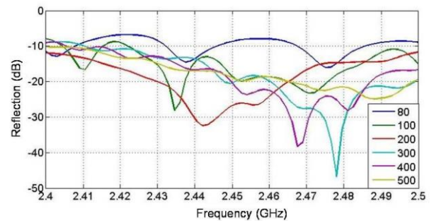
Fig. 6. Reflection coefficient for the proposed antenna depending on the diameter of the metallic duct (in mm).
