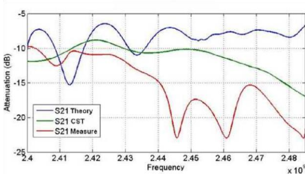
Fig. 2. Comparison of the transmission coefficient S21 in a metallic duct (diam. 200mm, length 3m) using waveguide theory, EM simulator or measurements.
