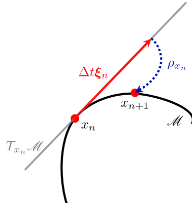
FIGURE 2. Optimization on a manifold \mathcal{M} : a retraction map \rho_{x_n} is used to project a tangential motion \Delta t \xi_n \in T_{x_n} \mathcal{M} from x_n \in \mathcal{M} back onto the optimization domain \mathcal{M} .
