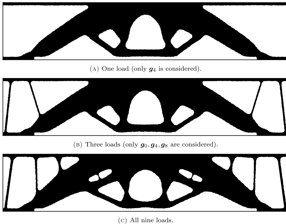
FIGURE 9. Optimized shapes for three possible configurations of the volume minimization problem subject to maximum compliance constraint (Sect. 6.2.1).
