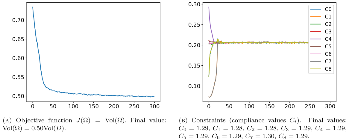
FIGURE 14. Convergence history curves for the nine load case of Section 6.2.1.
