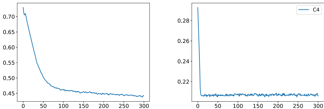
(A) Objective function J(\Omega) = \text{Vol}(\Omega) . Final value: \text{Vol}(\Omega) = 0.44\text{Vol}(D) . (B) Constraints (compliance values C_i ). Final values: C_4 = 1.29 .
