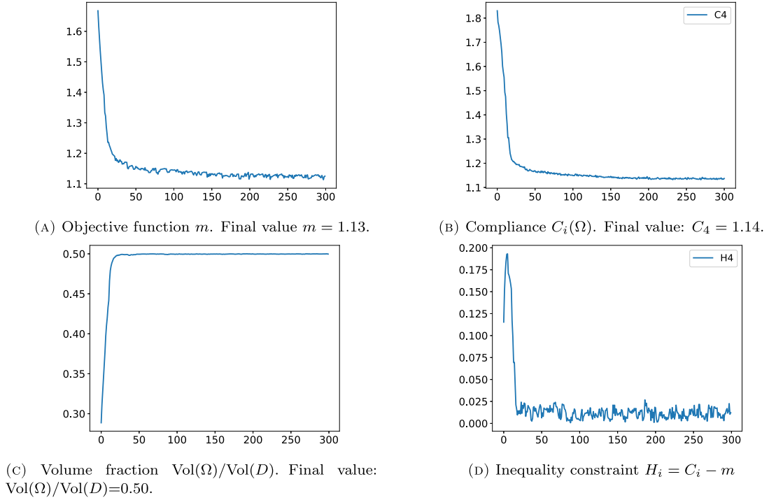
FIGURE 16. Convergence history curves for one load case of Section 6.2.2.
