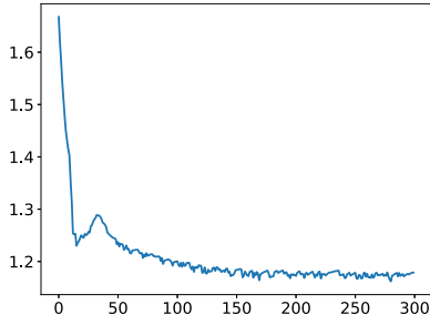
(A) Objective function m . Final value m = 1.18 .
