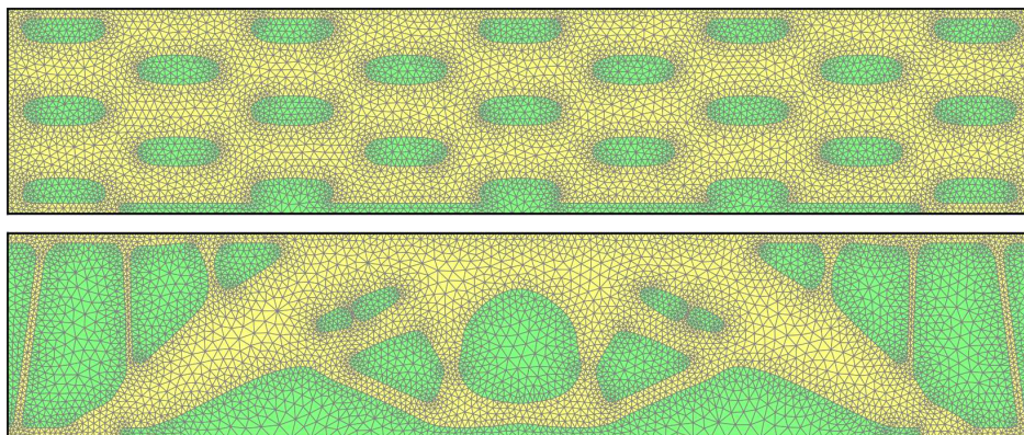
FIGURE 10. Meshes of the initial and final shapes for the nine load case of Figure 9c (Sect. 6.2.1).
