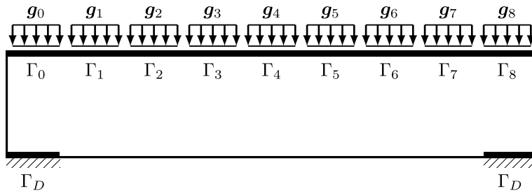
FIGURE 7. Geometric setting for the multiple load case test case.
