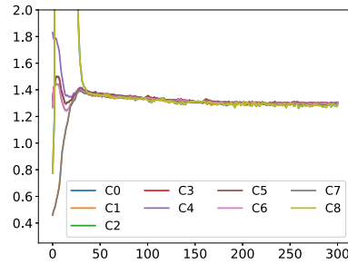
(B) Compliance values C_i(\Omega) . Final values: C_0 = 1.29 , C_1 = 1.29 , C_2 = 1.30 , C_3 = 1.31 , C_4 = 1.31 , C_5 = 1.31 , C_6 = 1.30 , C_7 = 1.29 , C_8 = 1.29 .
