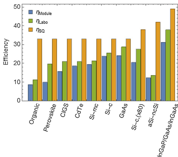
Figure 1. Best module (blue), best cell (green), and Shockley–Queisser (SQ) efficiency (yellow) of major technologies. Si-mc, Si-c, Si-c(x80), and aSi-ncSi stand for multicrystalline, crystalline, crystalline under 80 suns illumination and amorphous/nanocrystalline silicon, respectively. Data from [16,18].
