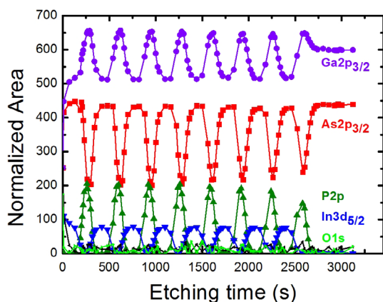
Figure 24. Time evolution during monoatomic \text{Ar}^+ etching of the XPS area of the peaks related to the elements constituting of the InGaAs/GaAsP multilayer stack.
