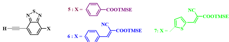
Figure 12. Schematic representation of the molecular formula of new acceptor building blocks 5–7 (protected form with TMSE = 2-(trimethylsilyl)ethyl).
