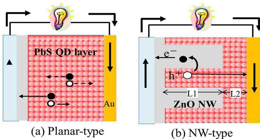
Figure 13. QD-based solar cells of two different types.
