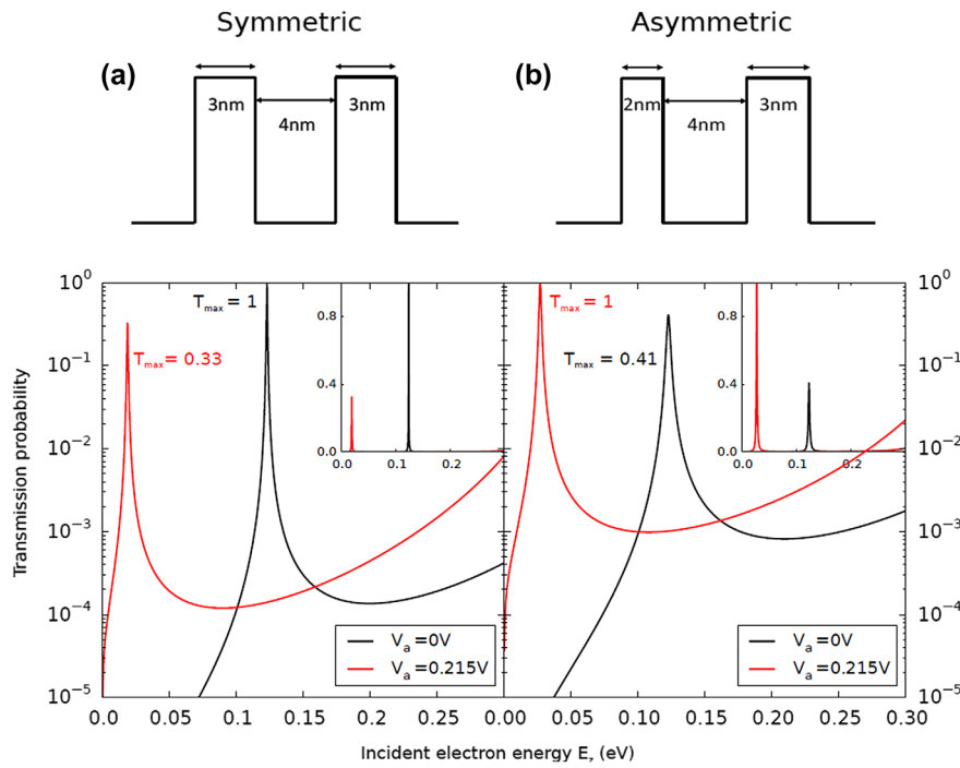
Figure 9. Modeled electronic transmissions of symmetric (a) and asymmetric (b) \text{Al}_{0.6}\text{Ga}_{0.4}\text{As}/\text{GaAs}/\text{Al}_{0.6}\text{Ga}_{0.4}\text{As} structures when no bias is applied (black curves) and under a 0.2 V bias (red curves). Inset: similar curves in linear scale (from [96]).
