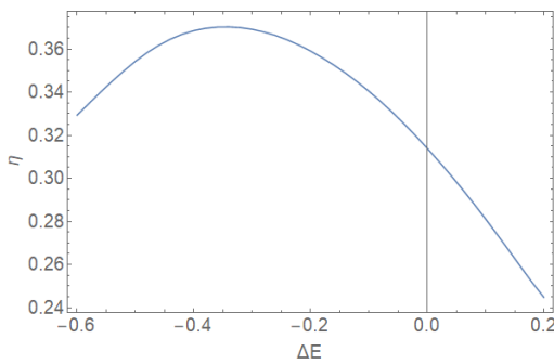
Figure 5 Power conversion efficiency as a function of the ratchet \Delta E in the ideal case with E_{g1} = 2 eV and E_{g2} = 1.1 eV.
