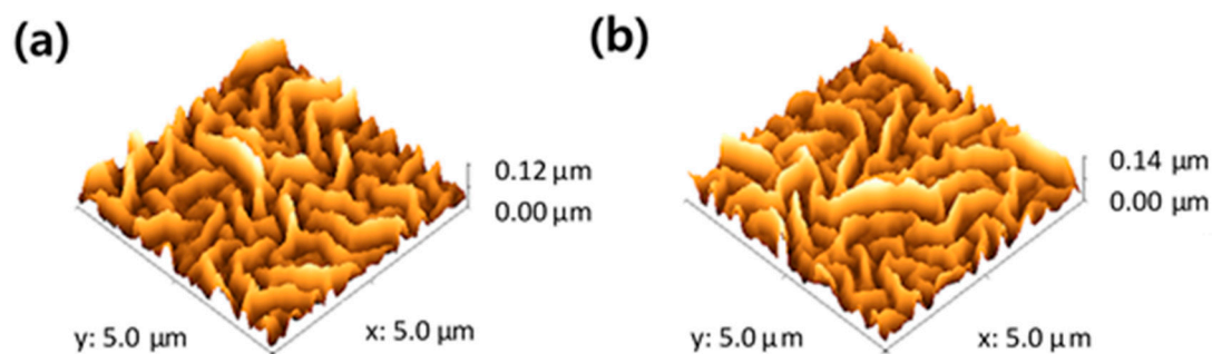
Figure 3. Atomic force microscopy (AFM) images of the ZnO nano-ripple, (a) the low temperature processed (10 min of drying time and annealing temperature of 150 °C) and (b) the ramping method.
