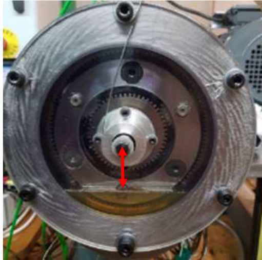
Fig. 3 Definition of oil sump static level (red arrow)
