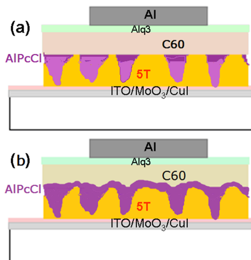
FIG. 8. Schematization of the geometrical section of PHJs with different intercalated AlPcCl layer thickness: (a) 10 nm, (b) 18 nm.
