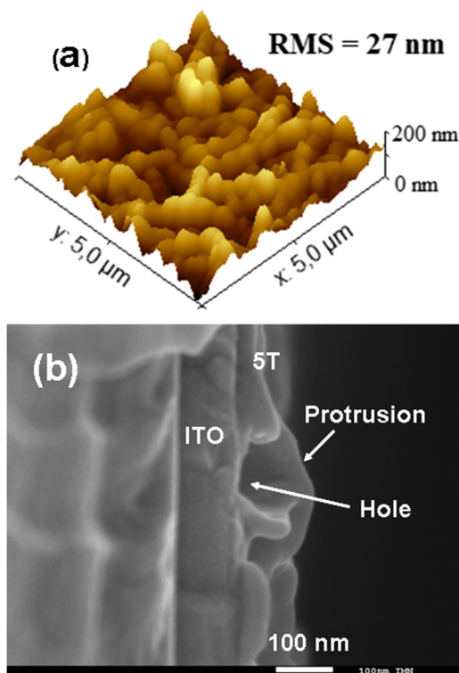
FIG. 6. 5T layer (Thickness measured by the quartz monitor: 60 nm), (a) AFM image, in 3D and (b) Cross section visualization of a structure Glass/ITO/MoO 3 /CuI/5T.
