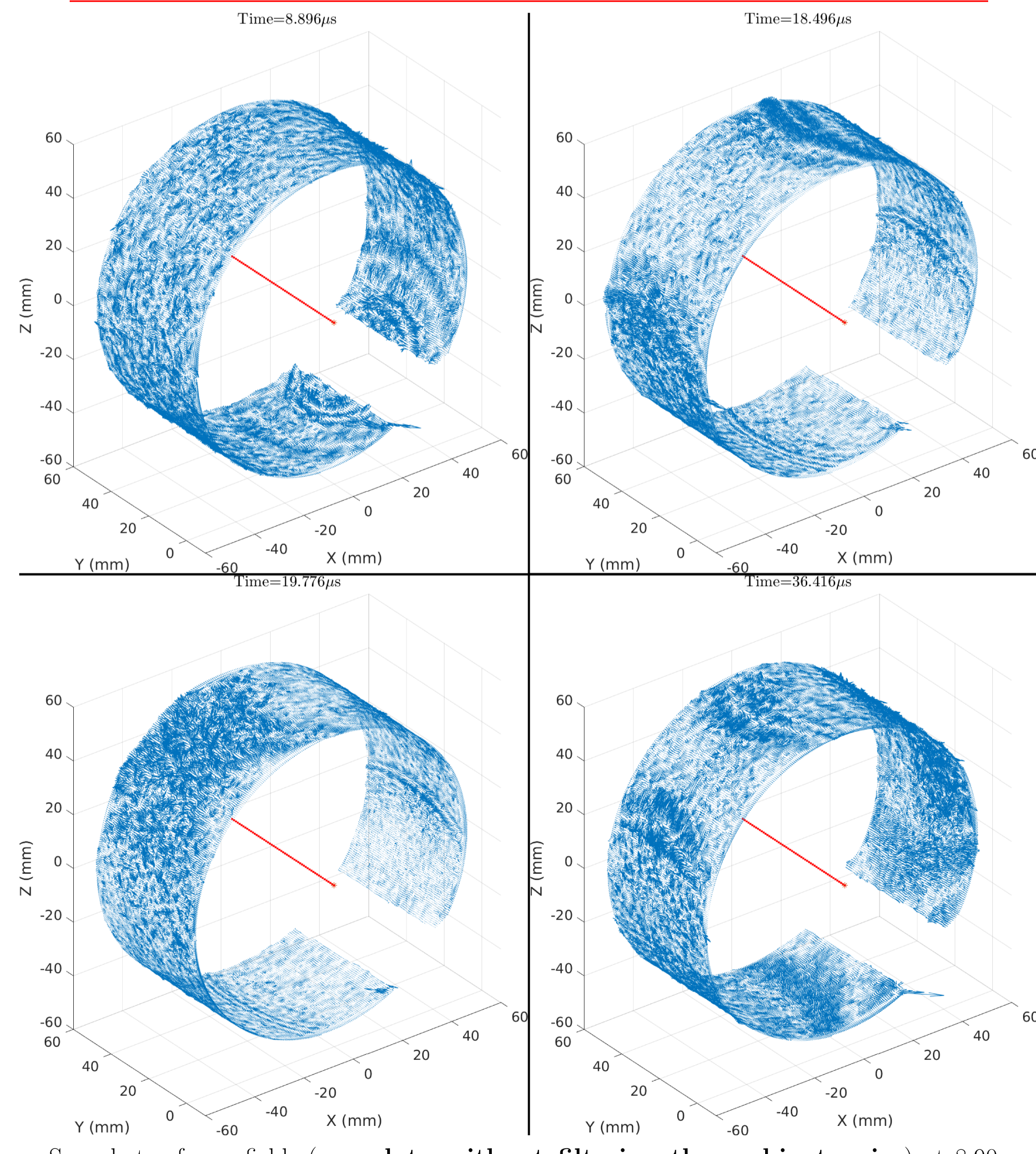
Snapshots of wavefields ( raw data without filtering the ambient noise ) at 8.90 \mu s , 18.50 \mu s , 19.78 \mu s and 36.42 \mu s , with the source at the middle of the gap. On the second snapshot we can clearly see the symmetric P wave fields in the front, followed by slower S waves. The different polarization of S waves are highlighted on the last one.
