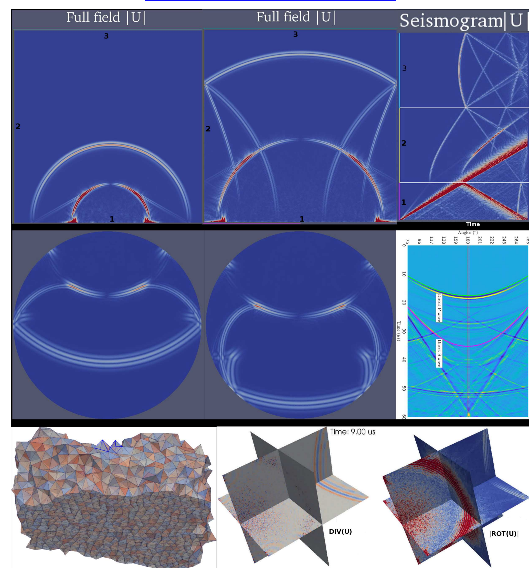
Corresponding 2D and 3D simulations by Finite Element method featured with IPDG[1]. The 3D simulation is performed in a reduced model with Absorbing Boundary Conditions due to memory limits.
