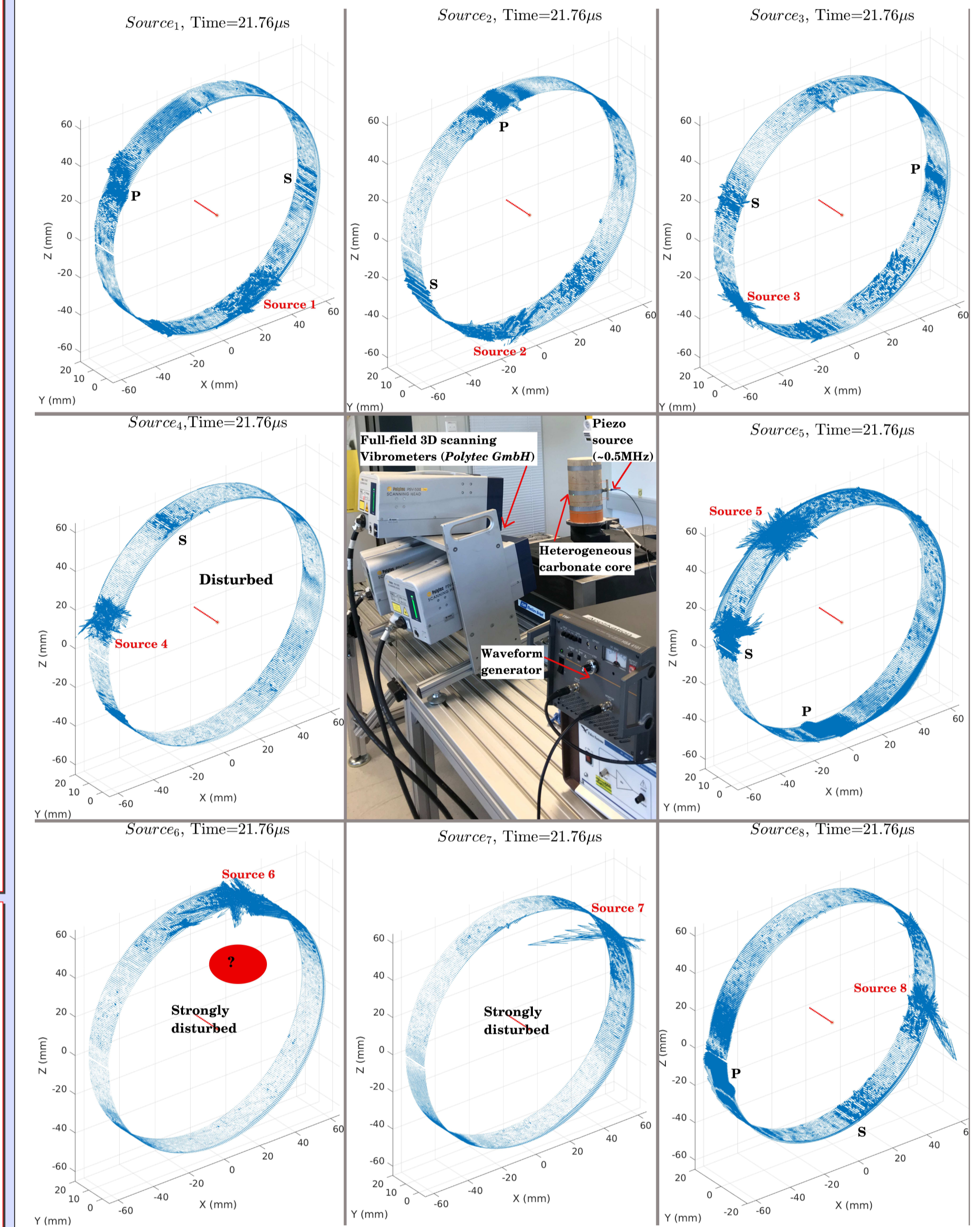
Snapshots at 21.76 \mu s for each source position. 8 uniformly distributed sources are deployed around the middle section of the core. Measurements close to the sources are not reliable because of instrumentation obstacles. The wavefield vectors are no longer symmetric in space due to the heterogeneities inside the natural rock. We can still recognize the P wavefield and S wavefield, however, they are strongly disturbed in the cases of source 6 and source 7, indicating probably an obstacle inside the core near these two sources.
