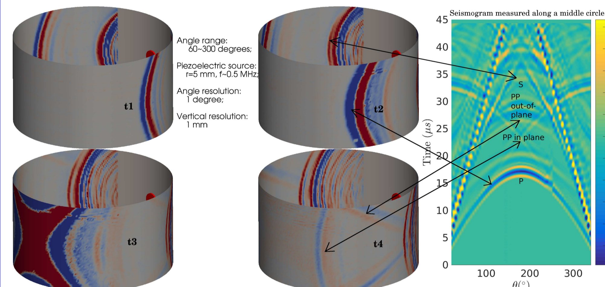
Radial components of displacements are measured. Snapshots and seismogram (around the mid-section) at/until t_1 , t_2 , t_3 , t_4 ( t_1 < t_2 < t_3 < t_4 ) are shown.
