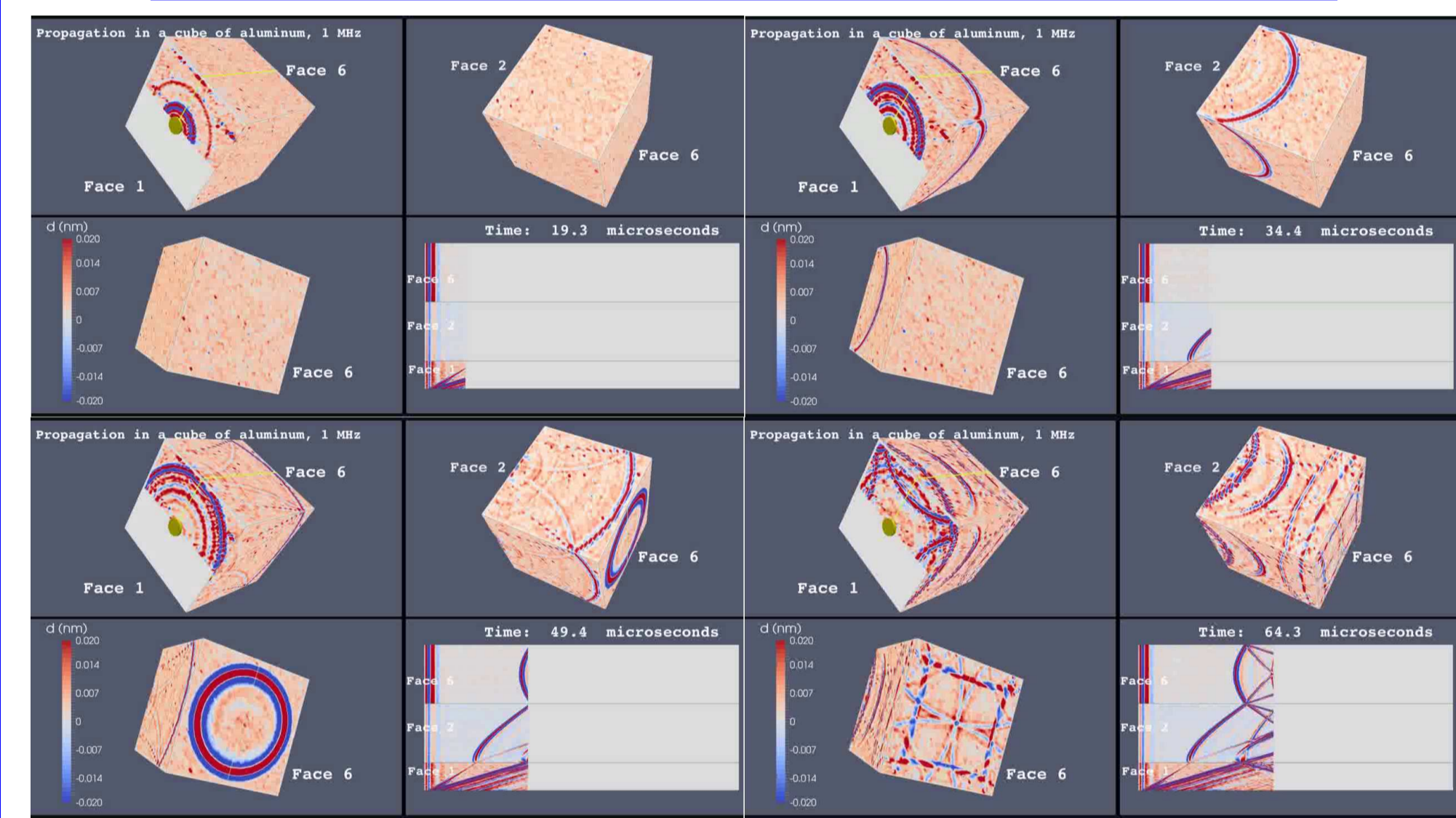
Normal components of displacements are measured on face 1 (source face), face 2 (upper face) and face 6 (opposite face). Snapshots and seismogram (along middle lines) at/until 19.3 \mu s , 34.4 \mu s , 49.4 \mu s and 64.3 \mu s are displayed.
