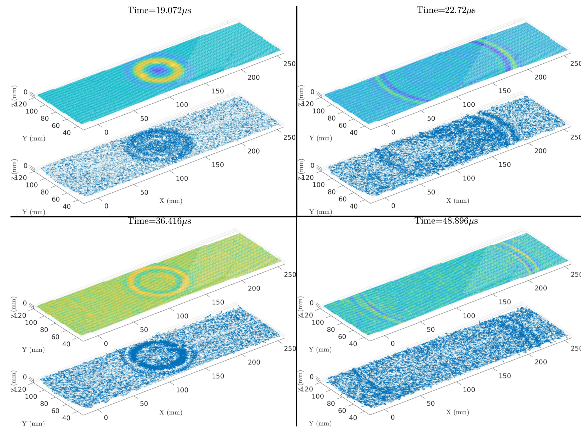
Snapshots of the displacements calculated by integrating the velocity measurements ( raw data without filtering the ambient noise ) at 19.07 \mu s , 22.72 \mu s , 36.42 \mu s and 48.90 \mu s . The first two are highlighted by P wave fields and the laser two by S waves. We can clearly see the different polarizations respectively for P and S waves.
