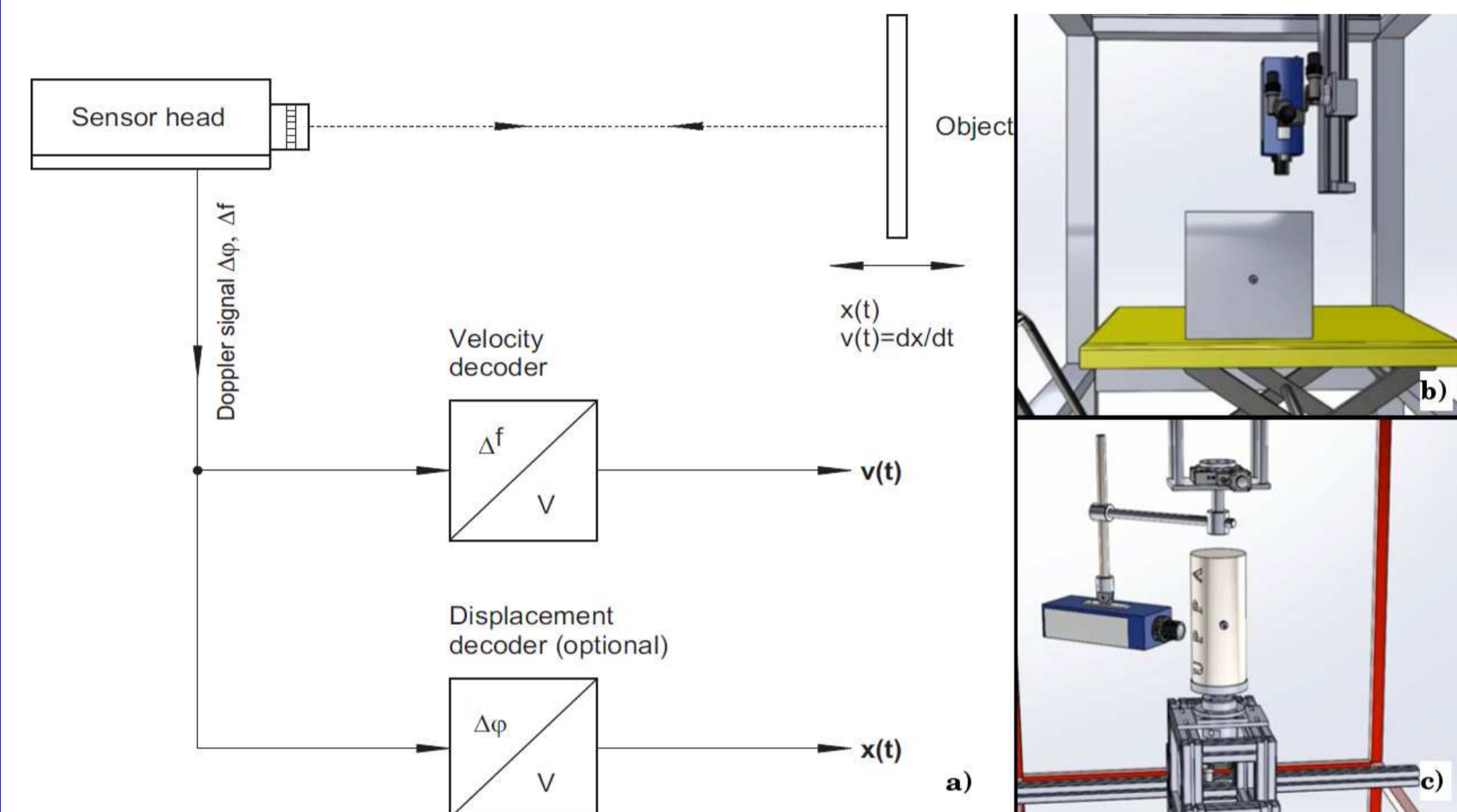
a) : Schematic view of the LDV principle; b) : Experimental setup of measurements on an Alu block by a single point LDV sensor. c) : Experimental setup for the Alu cylinder.
