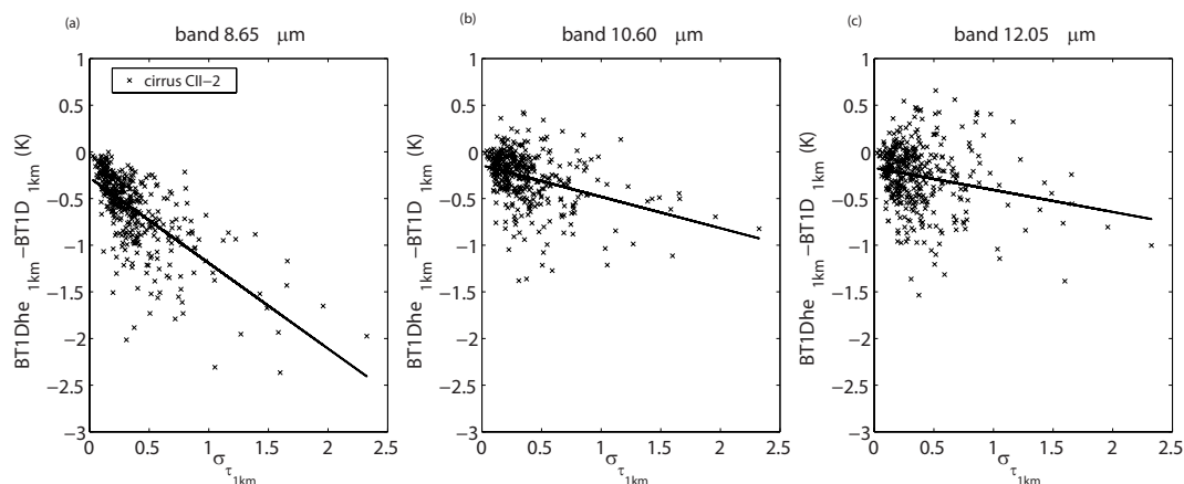
Figure 14. Differences between brightness temperatures viewed at the nadir between a 1-D radiative transfer with vertically heterogeneous columns ( BT1 - Dhe_{1\text{km}} ) and with homogeneous columns ( BT1 - D_{1\text{km}} ) as a function of the optical thickness standard deviation \sigma_{\tau_{1\text{km}}} for cirrus CII-2 and for the bands at 8.65 \mu\text{m} , 10.60 \mu\text{m} and 12.05 \mu\text{m} .
