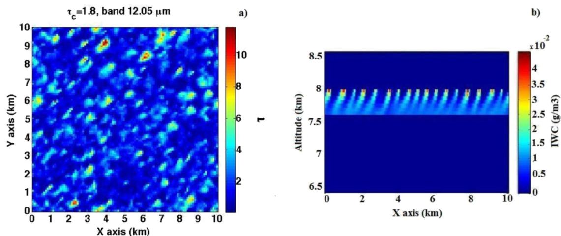
Figure 1. (a) 10 \text{ km} \times 10 \text{ km} optical thickness field at 12.05 \mu\text{m} with a horizontal spatial resolution of 100 \text{ m} ; (b) x-z view of the cirrus ice water content (IWC) with a vertical spatial resolution of 58 \text{ m} .
