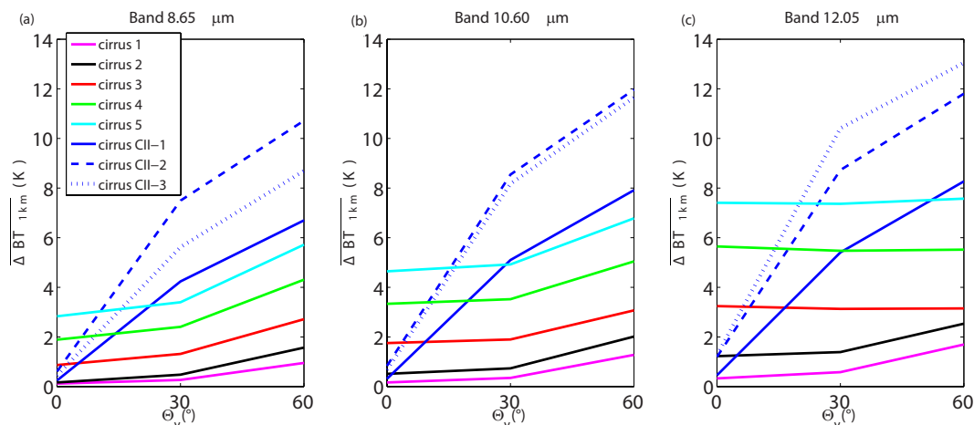
Figure 17. Mean difference \overline{\Delta BT}_{1\text{km}} as a function of the zenith view angle \Theta_v(^{\circ}) for cirrus 1 to 5 and cirrus CII-1 & CII-2 for the bands at 8.65 \mu\text{m} , 10.60 \mu\text{m} and 12.05 \mu\text{m} .
