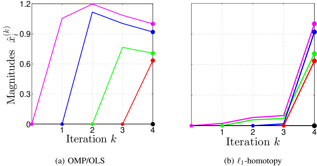
Fig. 2. Behavior of OMP and \ell_1 -homotopy in the case of a toy problem ( m = n = 5 ) corresponding to a 4-sparse noiseless representation. (a) The OMP and OLS iterates are identical and yield magnitudes \hat{x}_i^{(k)} with non-monotonous variations throughout the iterations k . (b) On the contrary, the magnitudes of the \ell_1 -homotopy iterates are always increasing. The ground truth magnitudes x_i^* are represented with bullets for k = 4 , and are exactly recovered after K = 4 iterations ( \hat{\mathbf{x}}^{(K)} = \mathbf{x}^* ).
