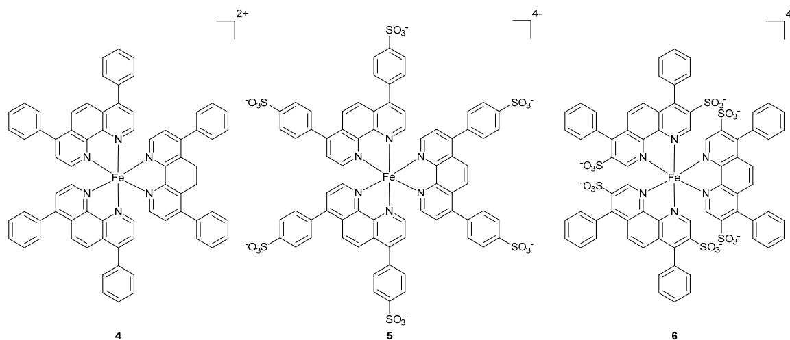
Figure 2. Chemical structures of the Fe(II) complexes investigated in this work. Complexes 4 was isolated as a PF 6 salt and the complexes 5 and 6 were isolated as Na salts.
