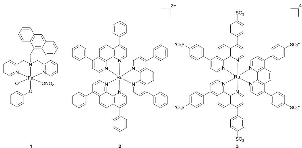
Figure 1. Chemical structures of a Fe(III) complex ( 1 ) investigated by Chakravarty and co-workers and Ru(II) bphen complexes ( 2 , 3 ) investigated by Glazer and co-workers as Photodynamic Therapy photosensitizers (PDT PSs).
