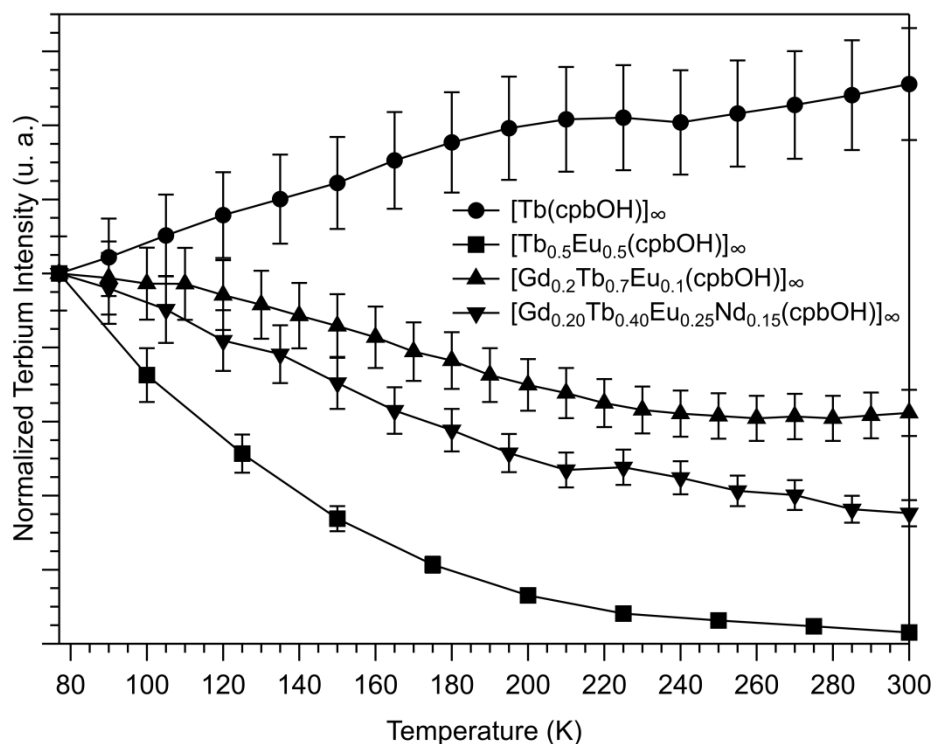
Figure 15. Tb(III) normalized luminescence intensities in [\text{Tb}(\text{cpbOH})]_{\infty} , [\text{Tb}_{0.5}\text{Eu}_{0.5}(\text{cpbOH})]_{\infty} , [\text{Gd}_{0.2}\text{Tb}_{0.7}\text{Eu}_{0.1}(\text{cpbOH})]_{\infty} and [\text{Gd}_{0.20}\text{Tb}_{0.40}\text{Eu}_{0.25}\text{Nd}_{0.15}(\text{cpbOH})]_{\infty} .
