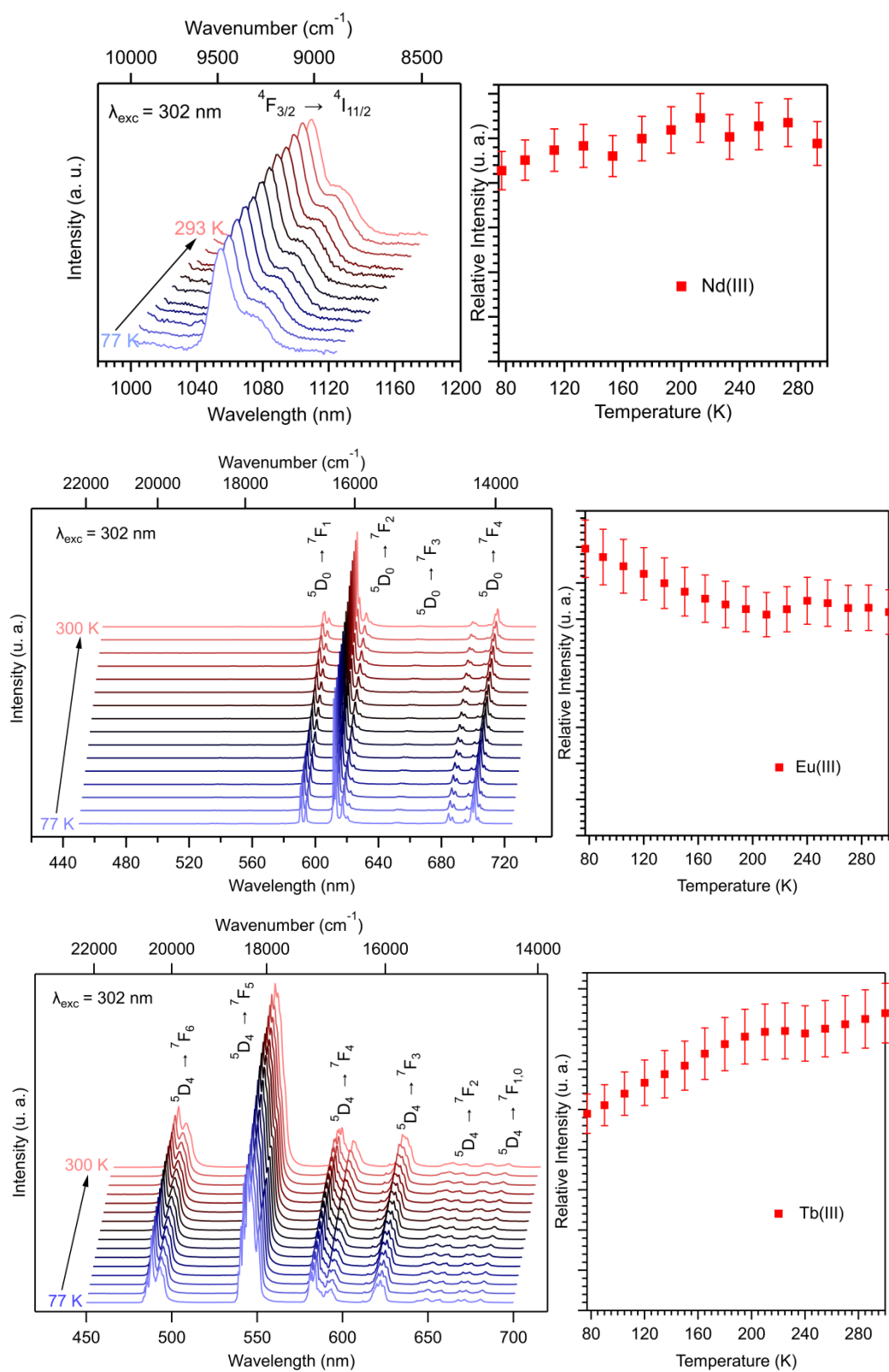
Figure 5. Left: Luminescence spectra versus temperature of [\text{Ln}(\text{cpbOH})]_{\infty} with Ln = Nd (Top), Eu (Middle) or Tb (Bottom). \lambda_{\text{exc}} = 302 \text{ nm} . Right: Integrated intensity I_{\text{Ln}} versus T for the three compounds.
