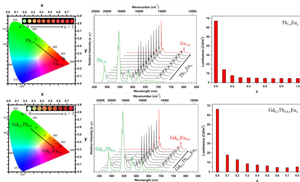
Figure 8. Colorimetric coordinates, luminescence spectra ( \lambda_{exc} = 303 \text{ nm} ) and luminance versus x under UV irradiation of [\text{Tb}_{1-x}\text{Eu}_x(\text{cpbOH})]_{\infty} with 0 \leq x \leq 1 (Top) and of [\text{Gd}_{0.2}\text{Tb}_{0.8-x}\text{Eu}_x(\text{cpbOH})]_{\infty} with 0 \leq x \leq 0.8 (Bottom).
