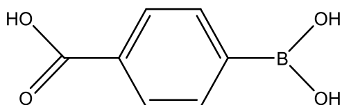
Scheme 1. Schematic representation of the 1,4-carboxyphenylboronic acid hereafter symbolized by Hcpb
