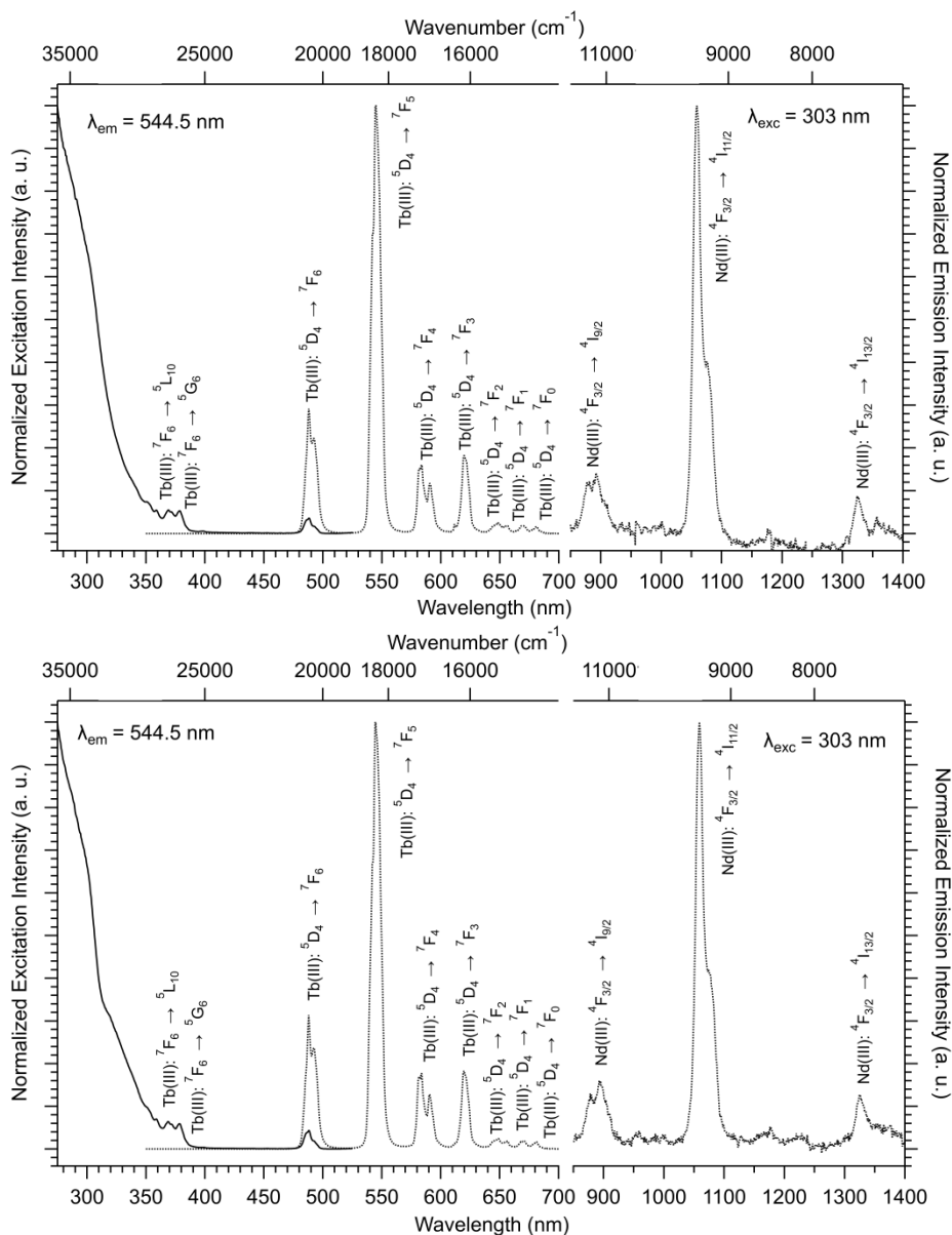
Figure 11. Solid state excitation and emission spectra of [\text{Tb}_{0.95}\text{Nd}_{0.05}(\text{cpOH})]_{\infty} (Top) and of [\text{Gd}_{0.2}\text{Tb}_{0.75}\text{Nd}_{0.05}(\text{cpOH})]_{\infty} (Bottom) at 293 K.
