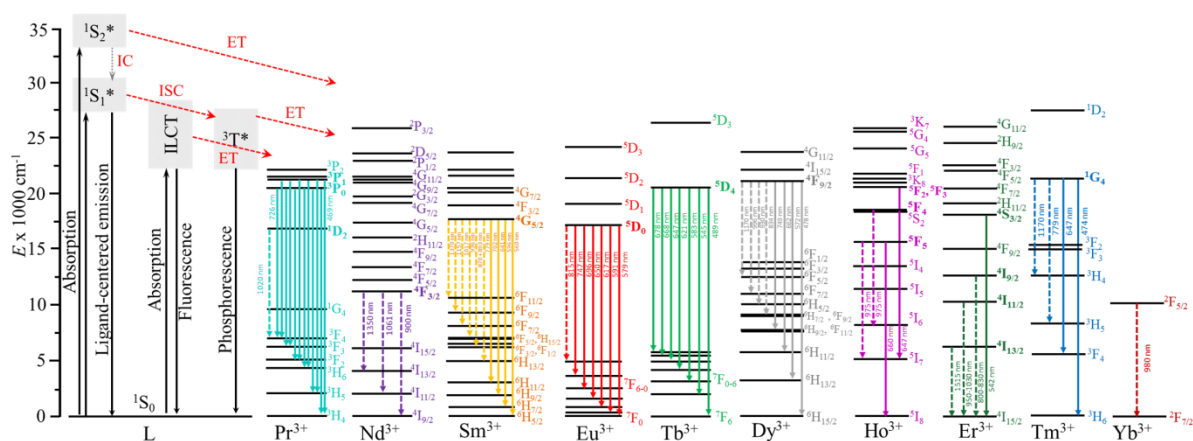
Scheme 3. Simplified Dieke-Jablonsky diagram for emissive lanthanide ions.
