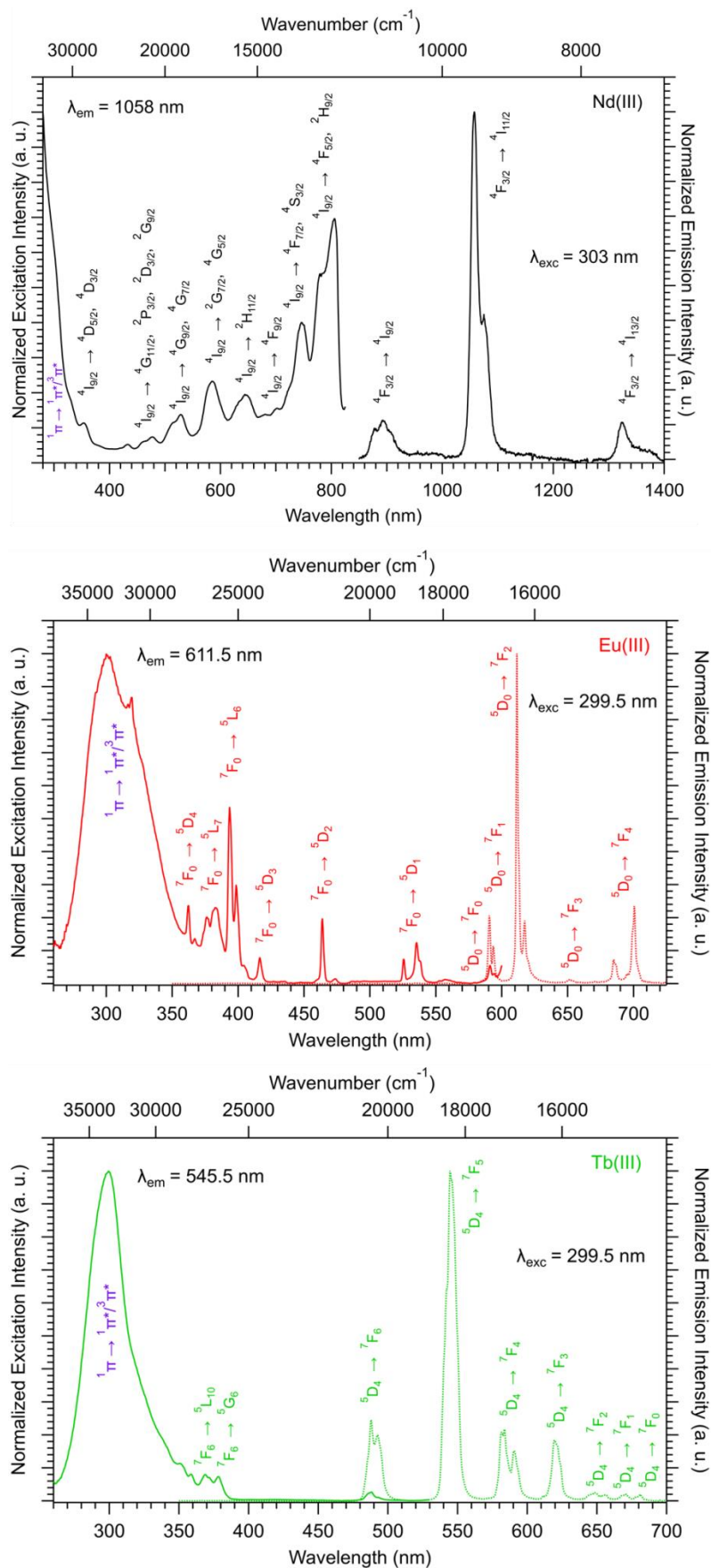
Figure 4. Solid state excitation and emission spectra of [\text{Ln}(\text{cpbOH})]_{\infty} with Ln = Nd(III), Eu(III) or Tb(III) at 293 K.
