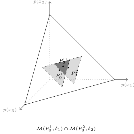
FIGURE 2. Example of conjunction.
