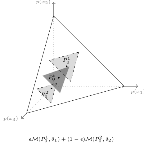
FIGURE 4. Example of PMM mixture.
