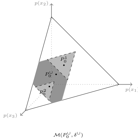
FIGURE 3. Example of approximated disjunction.
