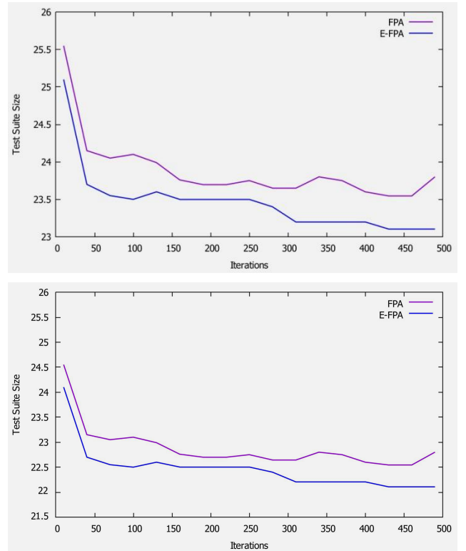
Figure 6: Convergence Rate of eFPA versus FPA for CA(N; 2, 10^5 ), and SCA(N; 20, 3)
