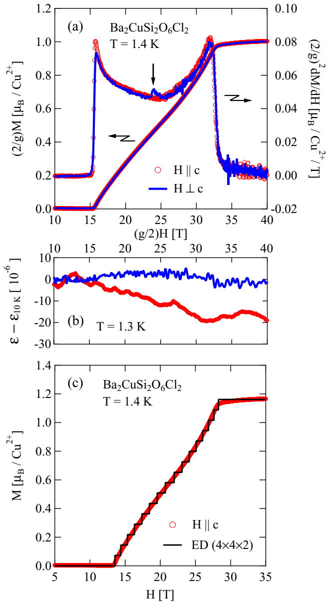
FIG. 4. (a) Magnetic-field dependence of magnetization M and its field derivative dM/dH for BCuSOC measured at 1.4 K for H \parallel c and H \perp c , which are normalized by the g factors. An arrow indicates an anomaly in dM/dH for H \perp c owing to a phase transition accompanied with a small magnetization jump. (b) Axial magnetostriction \varepsilon_a(H) , with H \perp c and H \parallel c , at T = 1.3 K after subtraction of the smooth background of similar magnitude measured at T = 10 K. The magnetostriction along and perpendicular to the c axis [at (g/2)H = 25 T] show magnitudes and signs which, in a magnetically isotropic system, would indicate conservation of the unit cell volume. (c) Comparison between experimental and theoretical magnetization curves for H \parallel c . The theoretical result was obtained using exact diagonalization (ED) for a 32-site spin cluster.
