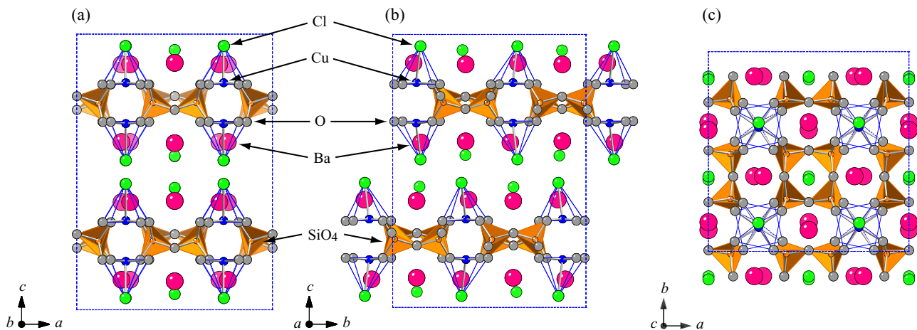
FIG. 1. Crystal structure of \text{Ba}_2\text{CuSi}_2\text{O}_6\text{Cl}_2 viewed along the (a) b , (b) a , and (c) c axes.
