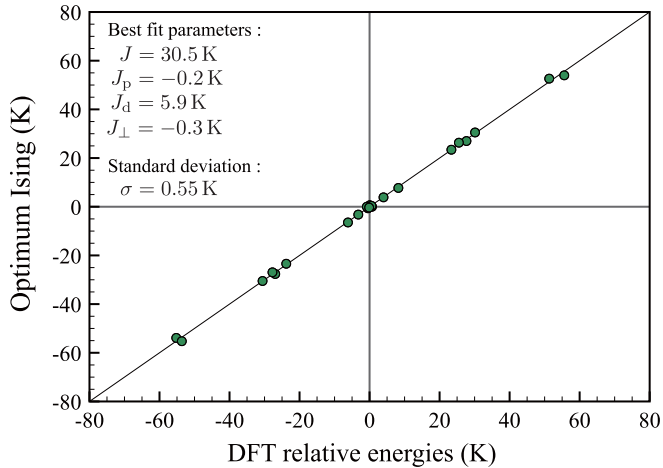
FIG. 7. Graphical representation of the results obtained by the least-squares fitting procedure employed to evaluate the magnetic couplings: optimized energies calculated with the Ising Hamiltonian (2) are represented as a function of the DFT + U_{\text{sef}} relative energies. Positive couplings correspond to AFM interactions according to Eq. (1).
