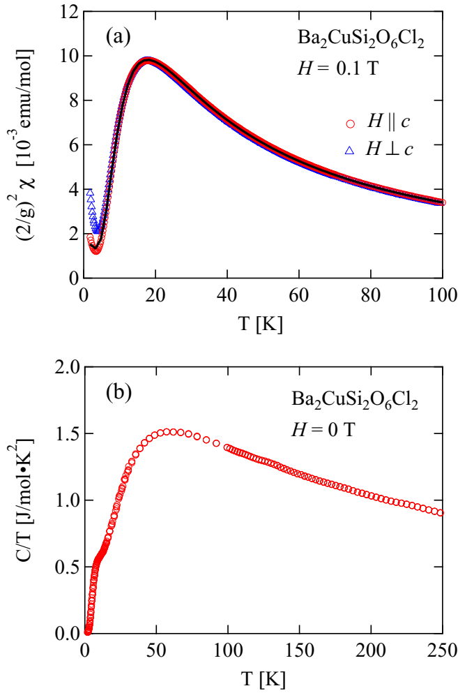
FIG. 2. (a) Temperature dependence of magnetic susceptibilities of BCuSOC measured for H \parallel c and H \perp c , which are normalized by the g factors of g_{\parallel} = 2.32 and g_{\perp} = 2.06 . The solid line denotes the fit obtained using Eq. (3). (b) Temperature dependence of total specific heat divided by the temperature measured at zero magnetic field.
