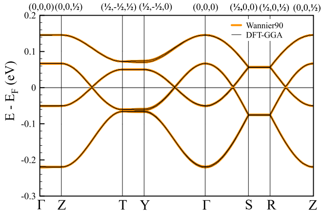
FIG. 5. Detail of the Cu- 3d_{x^2-y^2} band manifold around the Fermi level in \text{Ba}_2\text{CuSi}_2\text{O}_6\text{Cl}_2 calculated using paramagnetic GGA-PBE and interpolated with MLWFs.
