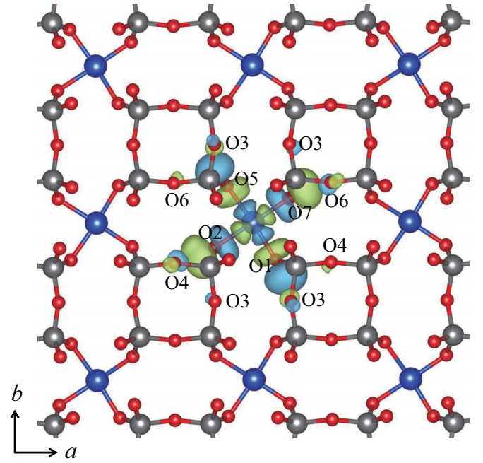
FIG. 6. MLWF centered on a Cu site. Large antibonding O-2p tails are clearly visible on the Cu coordinating oxygen atoms.
