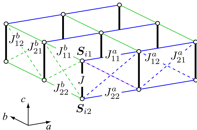
FIG. 3. 2D model of the exchange network in \text{Ba}_2\text{CuSi}_2\text{O}_6\text{Cl}_2 . Thick solid lines represent the intradimer exchange interaction J , and thin solid and dashed lines, respectively, represent the interdimer exchange interactions J_{\alpha\beta}^a and J_{\alpha\beta}^b ( \alpha, \beta = 1, 2 ).
