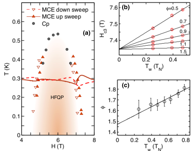
FIG. 7. (a) The solid black circles are the position of the anomaly from specific-heat measurements. The open red triangles indicate the position of the anomaly in temperature for fields being swept down, the solid red triangles are obtained from up sweeps. The dashed (solid) red line presents a characteristic temperature-field trace for sweeping the magnetic field down (up). (b) Determination of the critical field H_{c3}(0) by fitting the phase boundary H_{c3}(T) - H_{c3}(0) \propto T^\phi for various values of the critical exponent and different temperature windows. (c) Determination of the critical exponent \phi using the value of the critical field H_{c3} of 7.345 \pm 0.003 T found in (b).
