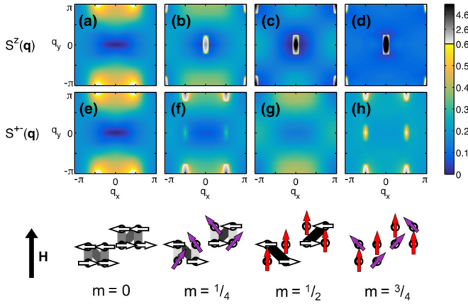
FIG. 9. Structure factor and magnetic order in NIT-2Py calculated by DMRG in the Brillouin zone of the square lattice for a cylinder of size L_x \times L_y = 32 \times 8 (see text). (a)–(d) Longitudinal and (e)–(h) transverse components of the spin structure factor for different values of magnetization m = 0, \frac{1}{4}, \frac{1}{2}, and \frac{3}{4} . The corresponding magnetic order is sketched below each column. Red spins align along the field direction, while violet spins have a component along the field direction and order in the plane transverse to the field. White/empty arrows represent spins in a rotational invariant quantum superposition for tetramers. The gray scale in the bonds indicates the relative strength of the correlations, with black representing a strong dimer.
