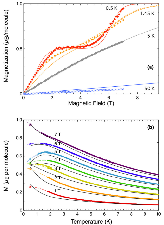
FIG. 3. (a) Magnetization of NIT-2Py as a function of the applied field. The data at 0.5 K are shown as solid diamonds, for 1.45 K as solid circles, for 5 K as filled squares, and for 50 K as open circles. The dashed line shows pulsed field magnetization at 1.43 K. The solid lines are obtained by minimizing the difference between the calculated magnetization obtained from diagonalizing Eq. (2) for a system of tetramers and the experimental results, as discussed in the last paragraph of Sec. IV. (b) Magnetization of NIT-2Py as a function of temperature. The filled symbols are the data taken with a VSM SQUID, and the open symbols were taken with the ^3\text{He} option. The solid lines are theoretical values calculated as described in (a).
