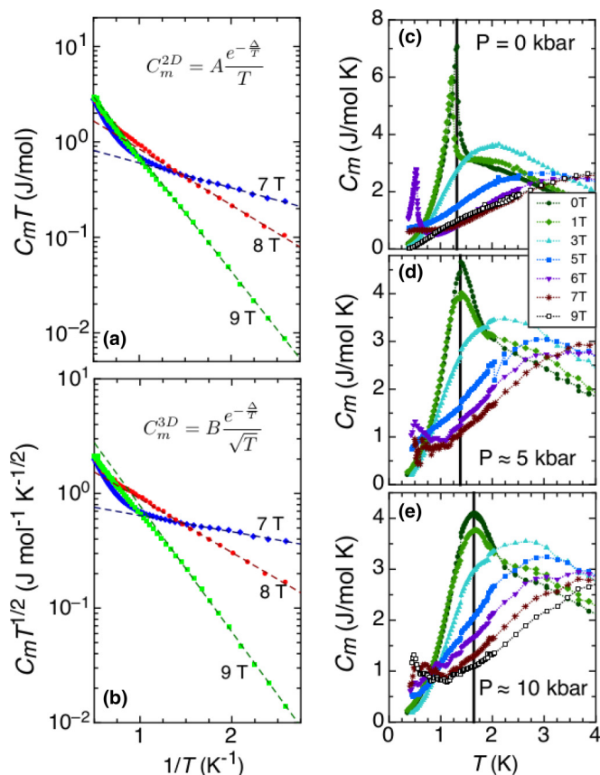
FIG. 8. (a) Semilogarithmic plot of the magnetic specific heat C_m of NIT-2Py presented as C_m T vs 1/T for 7 (diamonds), 8 (circles), and 9 T (squares). The dashed lines are fits to C_m^{2D} = A \frac{e^{-\Delta}}{T} expected for 2D magnons. (b) Same data as shown in (a), but shown as C_m \sqrt{T} vs 1/T . The dashed lines are fits to C_m^{3D} = B \frac{e^{-\Delta}}{\sqrt{T}} . (c) Magnetic specific heat C_m of NIT-2Py measured in a pressure cell at ambient pressure in the temperature range from 0.4 to 4 K. The solid line marks the position of the zero-field anomaly. (d) C_m data for an applied pressure of 5 kbar. (e) C_m data for 10 kbar of pressure.
