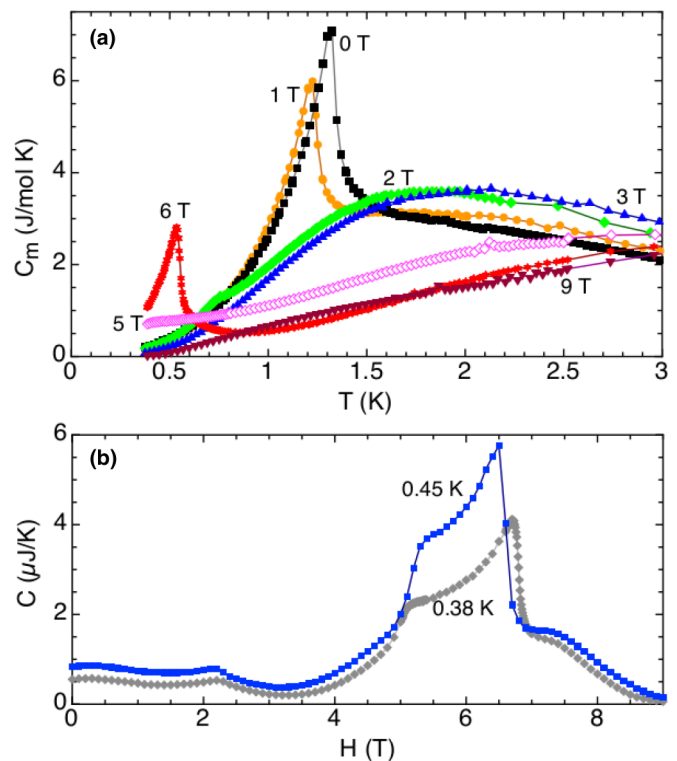
FIG. 5. (a) Magnetic contribution to the specific heat of NIT-2Py for various magnetic fields and temperatures from 0.35 to 3 K. The zero-field data shown as the solid squares show a peak at 1.32 K. A field of 2 T almost completely suppresses this phase transition shown as the solid green diamonds, and by 3 T, shown as solid blue triangles, all that is left of the transition is very broad anomaly centered at 2 K. The red solid diamonds show the data at 6 T, where we see a second sharp peak associated with a second phase transition. This transition is fully suppressed by 9 T. (b) Specific heat as a function of magnetic field measured at fixed temperatures. The data at 0.38 K, shown as solid diamonds, displays a first anomaly at about 2.2 T, followed by two more anomalies at 5.1 and 6.7 T.
