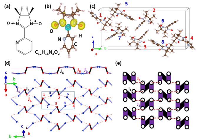
FIG. 1. Atomic and magnetic structure of NIT-2Py. (a) Structural formula. (b) Atomic structure and isosurfaces of positive (yellow) and negative (blue) spin density ( \pm 0.003 e/\text{\AA}^3 ). Oxygen atoms are represented in red, carbon atoms in brown, nitrogen atoms in gray, and hydrogen atoms in light pink. (c) Monoclinic unit cell. (d) Lateral and top view of the 2D arrangement of the three leading magnetic interactions in the (-1,0,2) plane: J_4 (black), J_6 (red), and J_9 (violet). The circles represent the C atom in the central O-N-C-N-O branch and the numbers correspond to those in (c). The solid lines outline a unit cell. (e) Topologically equivalent network of the magnetic lattice used for the DMRG calculations.
