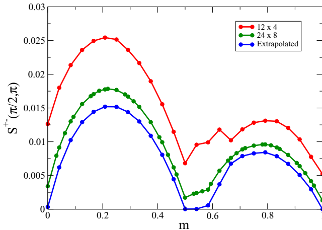
FIG. 10. Transverse structure factor S^{+-}(\pi/2, \pi) for two system sizes with the same aspect ratio, N = L_x \times L_y = 12 \times 4 and 24 \times 8 . Results in the thermodynamics limit were obtained through a linear extrapolation in 1/N . Numerical errors are smaller than the symbol size.
