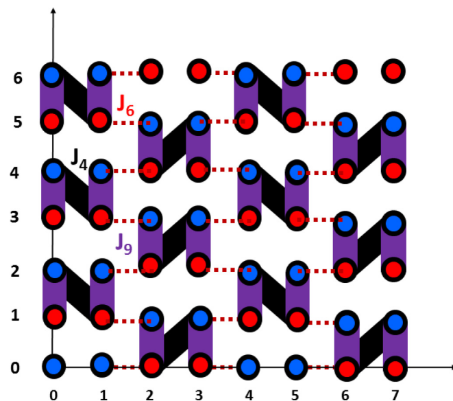
FIG. 11. Antiferromagnetic Néel order compatible with the calculated exchange interactions.
