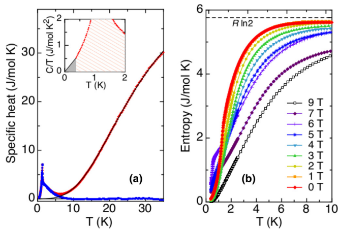
FIG. 4. (a) The measured specific heat C_p of NIT-2Py in zero magnetic field, the phonon contribution from the lattice C_{ph} , and the magnetic contribution C_m = C_p - C_{ph} are shown in black (solid line), red (diamonds), and blue (circles), respectively. The inset shows the linear extrapolation of C_p/T to zero temperature used to calculate the entropy. (b) Entropy associated with the phase transition in various magnetic fields for temperatures up to 10 K. The dashed line marks S = R \ln 2 , the value expected for a S = \frac{1}{2} per molecule.
