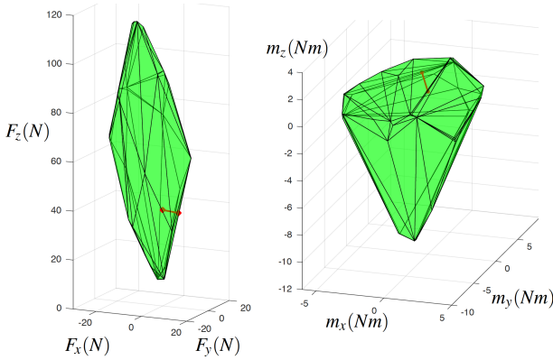
Fig. 9: Achievable wrench space of the eight quadrotor, eight cable ACTS evaluated at \mathbf{w}_{moment} = [0 \ 0 \ 0]^T Nm (left) and at \mathbf{w}_{force} = m_p \mathbf{g} N (right).
