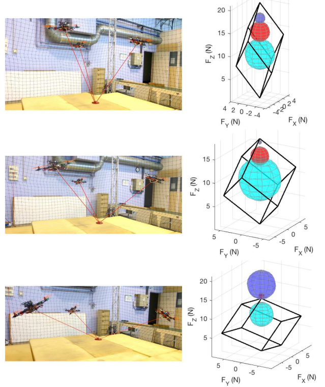
Fig. 13: The available wrench set of the ACTS prototype at \theta = 35^\circ (top), 50^\circ (middle) and 65^\circ (bottom) under quasi-static motion. The cyan, red and blue spheres are centered at \mathbf{w}_e = -m_p \mathbf{g} for payload masses of 1.0 kg, 1.5 kg and 1.8 kg respectively and have radius corresponding to the magnitude of their respective capacity margins.
