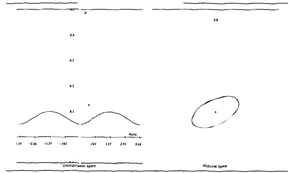
Fig. 3 An example Poincaré surface
