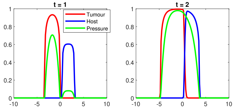
FIGURE 2. Solutions to (1) and corresponding pressure in the presence of vacuum. The system is initialised with two indicator functions with supports at a positive distance. The densities remain segregated, in agreement with known results on segregated solutions (see, e.g. , [8]).
