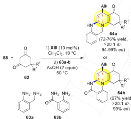
Scheme 18. Synthesis of 64a-b through secondary-amine catalyzed Michael addition followed by iminium ion trapping with a heteroatomic nucleophile. [38c]
