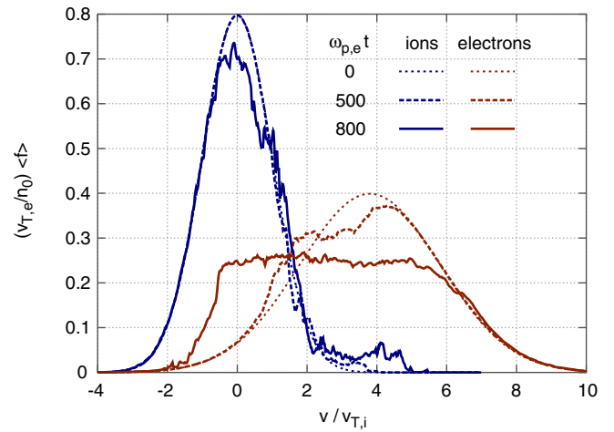
Figure 1. Snapshots of the velocity distributions in a Vlasov simulation of subcritical instability. Simulation parameters are v_d/v_{T,i} = 3.8 , e\phi/T \approx 0.2 and N_x \times N_v = 768 \times 8192 .
