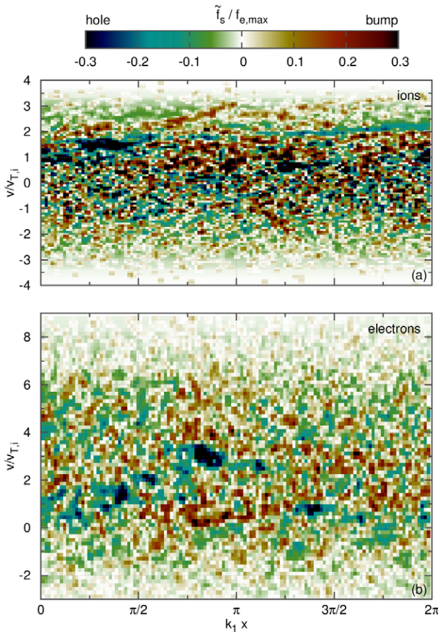
Figure 6. Snapshot at \omega_{p,e}t = 400 of the phase-space in the N_p = 102\,400 , full- f PIC simulation of figure 5 ( v_d/v_{T,i} = 2.5 ).
