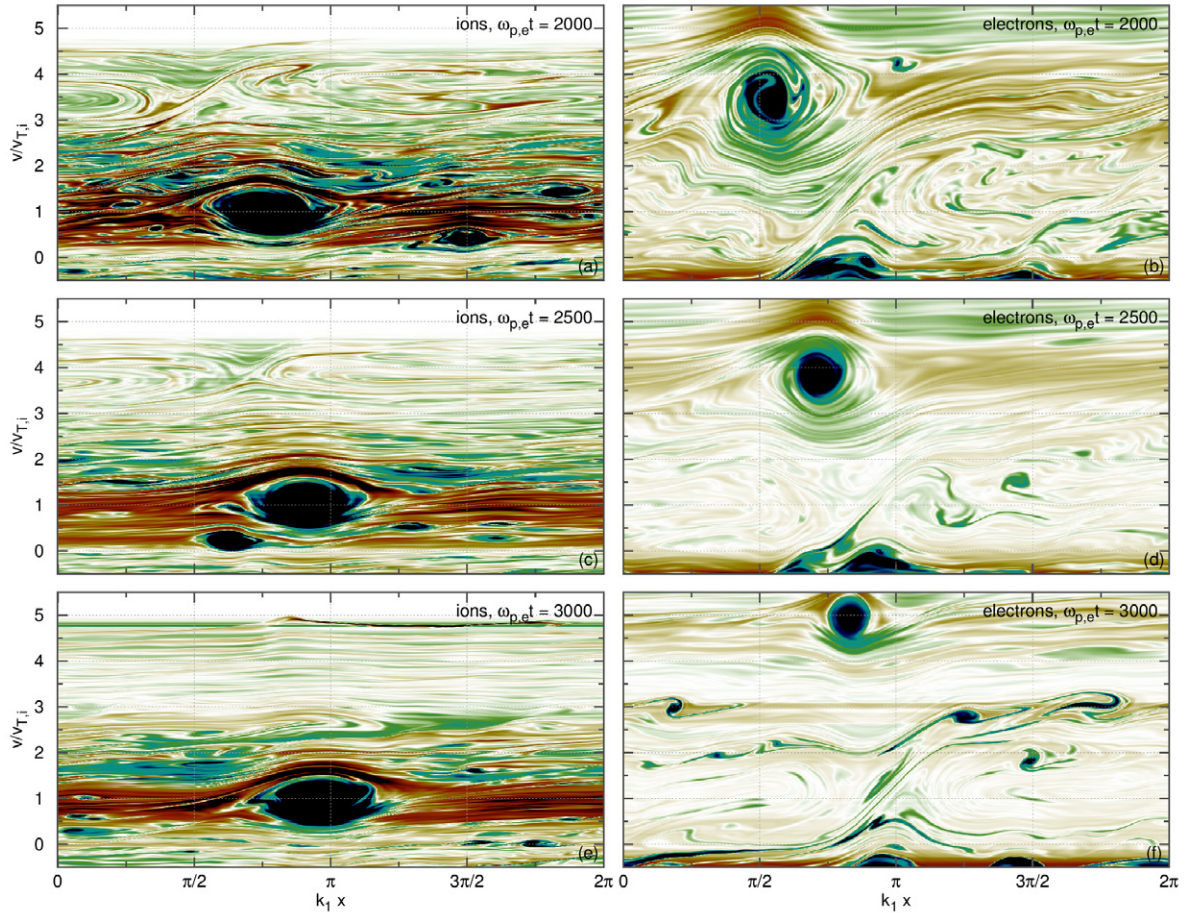
Figure 10. Same as figure 9, but for later times. Values of \omega_{p,e}t from top to bottom are 2000, 2500 and 3000.
