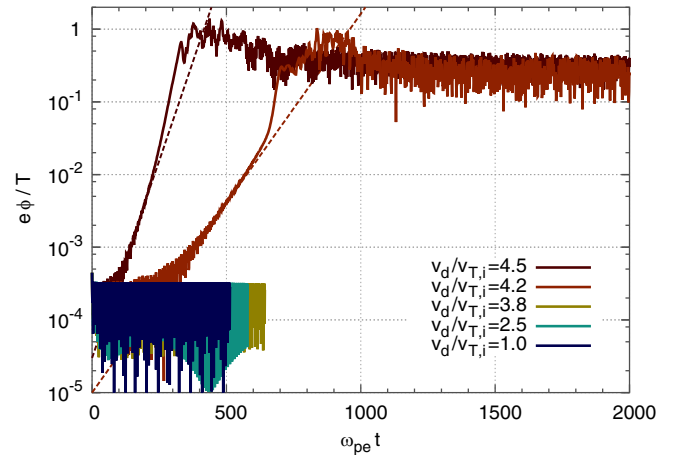
Figure 2. Time-evolution of the normalized potential energy in Vlasov simulations for small, incoherent initial perturbation, e\phi/T \approx 2 \times 10^{-4} . Linear theory is shown as dashed lines.
