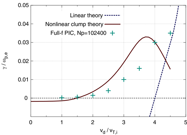
Figure 7. Growth rate of electron hole. Crosses: \gamma_{NL} measured in full- f PIC simulations with N_p = 102\,400 . Solid curve: nonlinear instability theory of [41].
