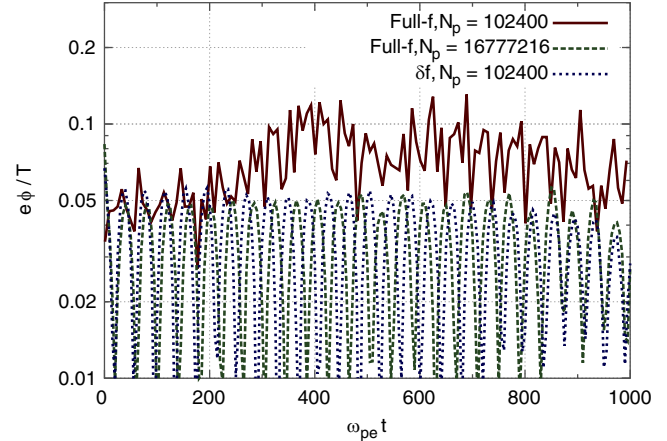
Figure 5. Time-evolution of the normalized potential energy in PIC simulations for v_d/v_{T,i} = 2.5 .
