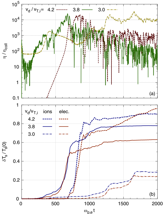
Figure 4. Time-evolution of (a) anomalous resistivity, normalized to \eta_{coll} = 10^{-7} m_e \omega_{p,e} / (n_0 q_i^2) , and (b) mean thermal energy perturbation. Three cases are shown, the simulation of figure 1 ( v_d/v_{T,i} = 3.8 , solid curves), a linearly unstable case ( v_d/v_{T,i} = 4.2 , dashed curves), and the reference case S of figure 16 ( v_d/v_{T,i} = 3.0 , chained curves).
