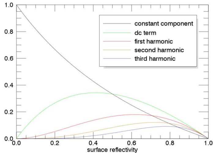
Figure 4. Amplitude of the Fourier components for a Fabry Perot interferometer, vs the reflectivity of the surfaces of the cavity. In a two-wave interferometer, there would be only the dc term and the fundamental frequency: we can see that for reflectivity about 30%, the Fabry-Perot interferometer is close to a two-wave interferometer, with a transmission about 55% and an intrinsic fringe contrast of 60%.
