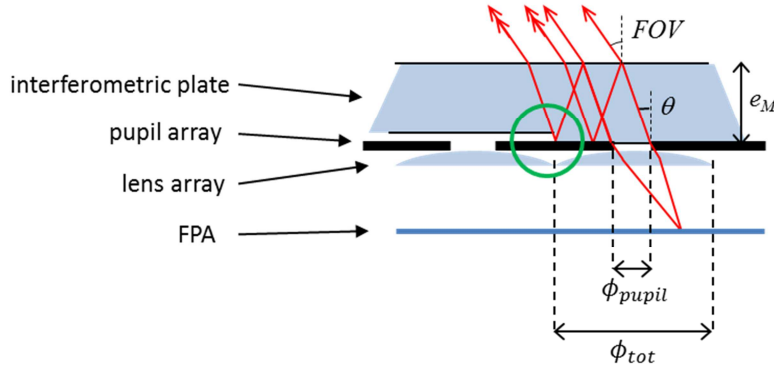
Figure 6. Upper limit for the field-of-view before cross-talk between two contiguous steps. In red, we have drawn rays from the FPA toward the scene. If we increase the field-of-view, then the marginal ray after one round-trip will be reflected by the neighbouring step (emphasized by the green circle).
