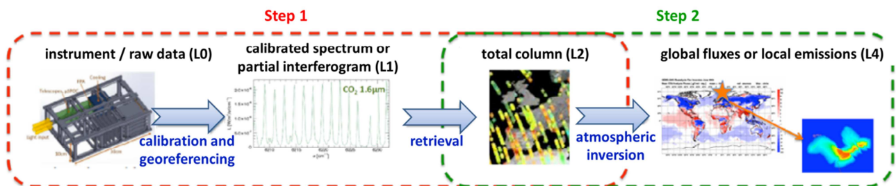
Figure 8. Level products. In GHG space missions, the target variable (surface fluxes, and in particular emissions – so-called L4 products) is not what is retrieved (total atmospheric columns XCO 2 – L2 products) from the observations (radiances – L1 products). A two-step approach is thus needed. First, after radiometric calibration, radiances measured by the instrument are interpreted in terms of total column, together with associated uncertainty and vertical sensitivity (which gives the contribution of each atmospheric layer to the total column). This step relies on an iterative loop between forward and inverse radiative transfer models. In a second step, the total columns are used to infer surface sources and sinks and their associated uncertainties through an atmospheric inversion, which usually relies on an atmospheric transport model.
