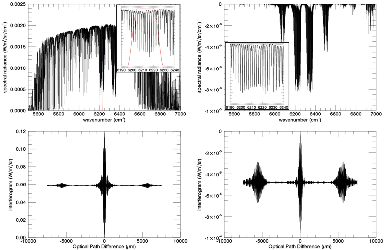
Figure 2. Typical radiance simulated with Modtran for a spaceborne mission viewing at nadir. Top: spectra; bottom: corresponding interferograms after filtering between 6200 cm -1 and 6225 cm -1 (red curve). Left: total radiance with a CO 2 concentration of 400 ppm; right: difference between the radiance with 405 ppm and with 400 ppm of CO 2 , the other parameters being unchanged.
