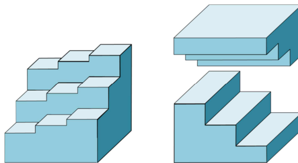
Figure 5. Two examples of possible geometry for the interferometric plate. On the left, it is made inside one material, with only one side engraved with a two-dimensional pattern. On the right, the cavity is formed between the inner sides of two plates each engraved with a one-dimensional pattern.
