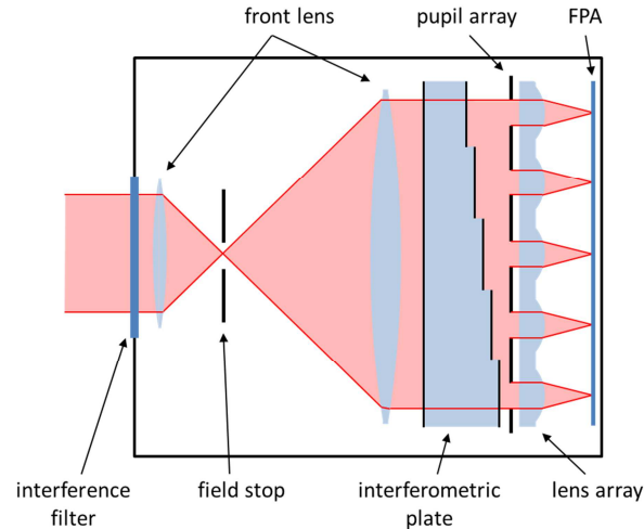
Figure 1. Optical principle of Nanocarb: a front afocal lens with a field stop is located before the core of Nanocarb, consisting in the interferometric plate and the lens array. Light is then focused on the FPA to obtain a set of images, each one being associated to one thickness of the interferometric plate.
