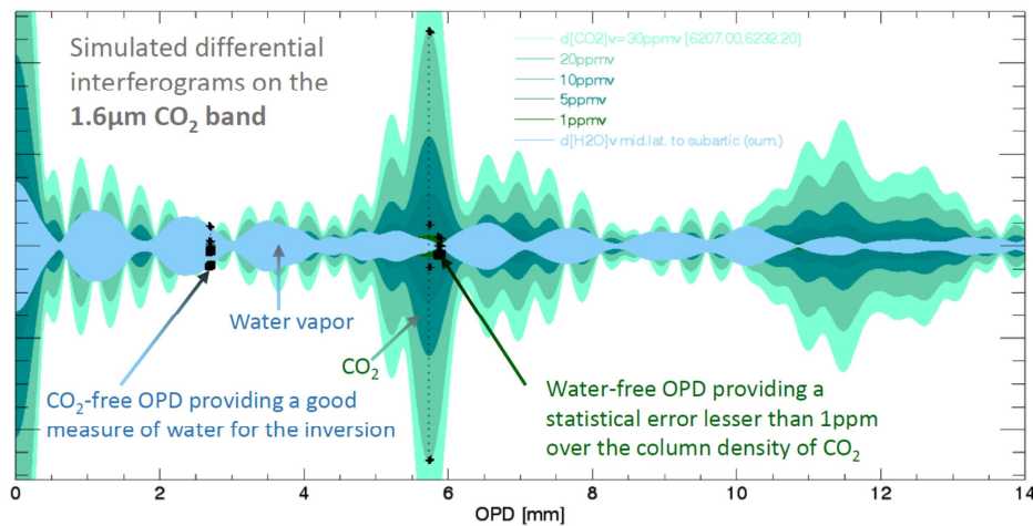
Figure 3. Jacobian interferograms (arbitrary unit) when varying the CO 2 or H 2 O concentration 13 . During the design phase of Nanocarb, the choice of the measured OPD will be done taking into account the impact of other species than CO 2 .
