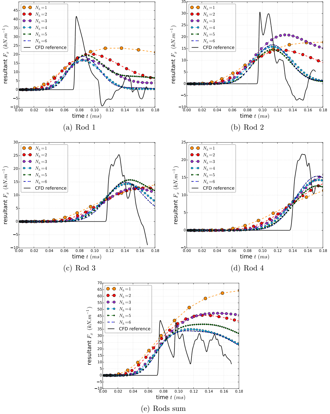
Figure 22: Resultant pressure force F_x(t) using the integral approach with different coarse meshes and the 1 st -order approximation of the wall pressure – comparison with the CFD reference (black line).
