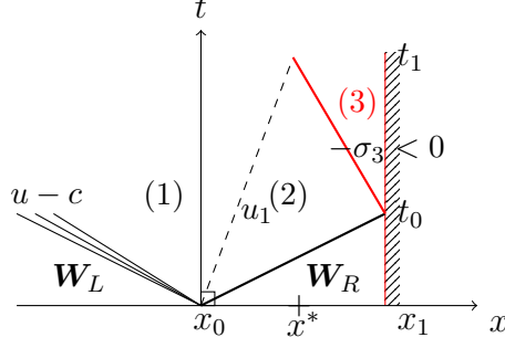
Figure C.31: Interaction of the reflected shock wave with the initial contact discontinuity (subsonic case: u_1 - c_1 < 0 ).
