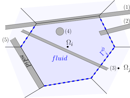
Figure 3: A (blue) control volume \Omega_i includes (gray) obstacles numbered from 1 to 5. Obstacles may: overlap part of the boundary of \Omega_i (1); partially occupy fluid cell (2); fully cross \Omega_i and halve it (3); be totally included in \Omega_i (4); or be aligned with part of the boundary of \Omega_i (5). The dashed blue surface corresponds to the fluid part \Gamma_i^\phi of the boundary of \Omega_i .
