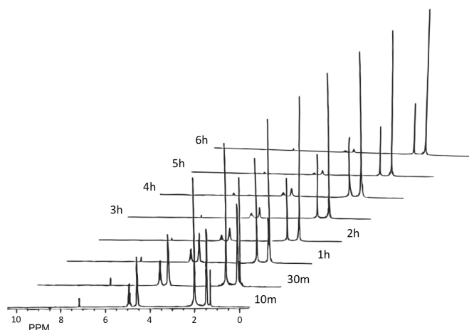
Fig. 1 Time evolution of the ^1\text{H} NMR spectrum for the reaction (\text{Me}_5\text{C}_5)_2\text{Yb} with buta-1,2-diene in \text{C}_6\text{D}_6 at 20^\circ\text{C} .
