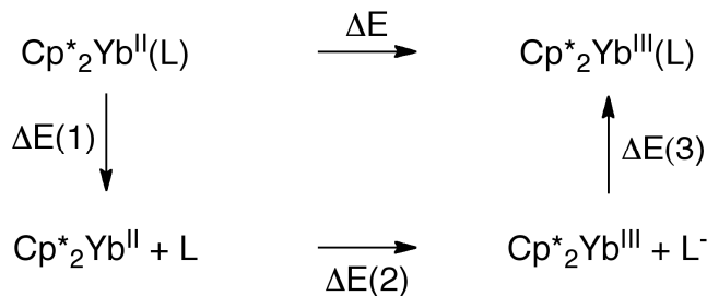
Scheme 1 A Hess cycle to determine the SET energy ( \Delta E ) using DFT methods.
