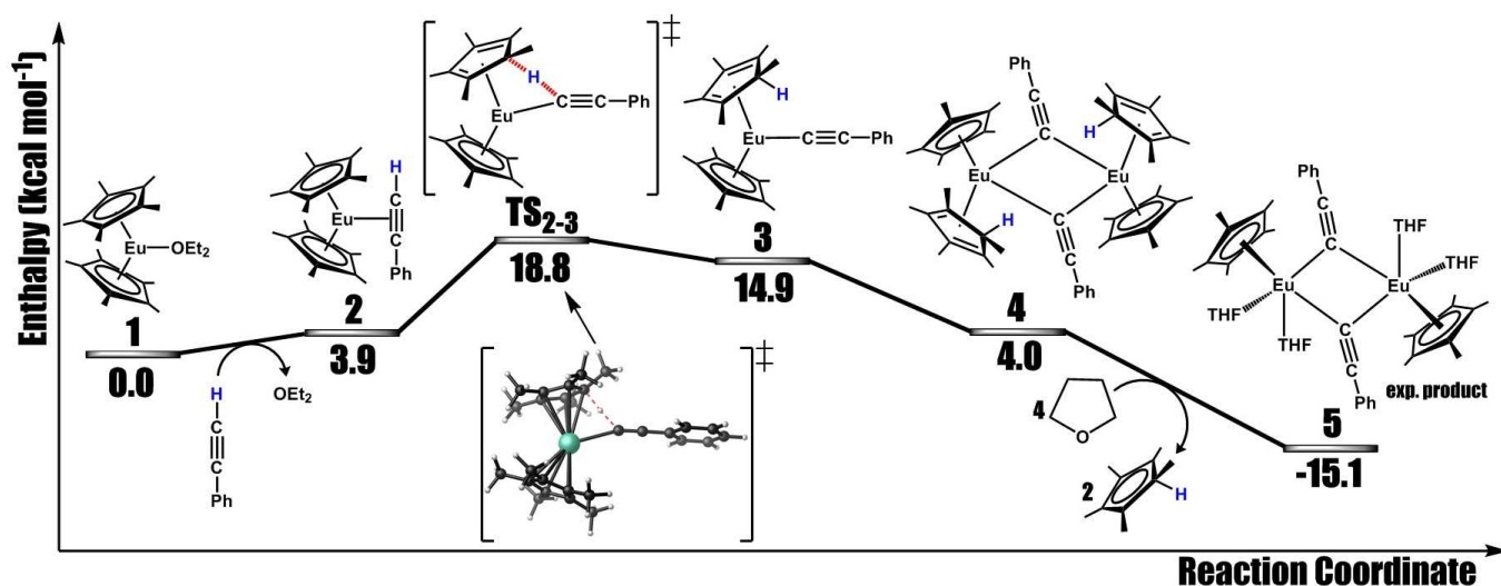
Fig. 3 B3PW91 enthalpy profile for the reaction mechanism of phenylacetylene with (Me 5 C 5 ) 2 Eu(OEt 2 ) in THF.
