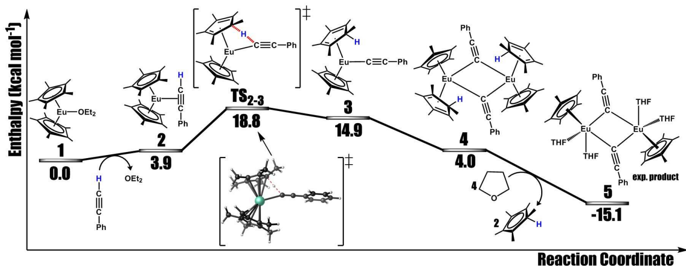
Fig. 3 B3PW91 enthalpy profile for the reaction mechanism of phenylacetylene with (\text{Me}_5\text{C}_5)_2\text{Eu}(\text{OEt}_2) in THF.
