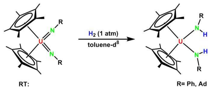
Scheme 2 Experimental net reaction of H_2 with (Me_5C_5)_2U(NR)_2 , with R = phenyl or adamantyl.
