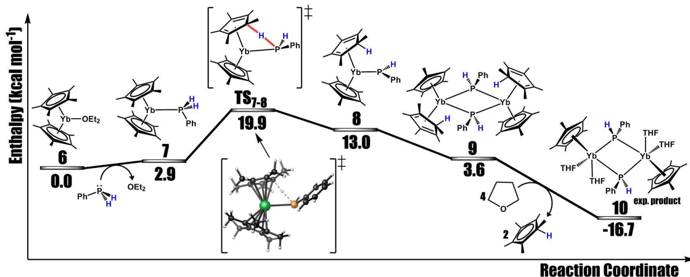
Fig. 4 B3PW91 enthalpy profile for the reaction mechanism of C_6H_5PH_2 with (Me_5C_5)_2Yb(OEt_2) in THF.
