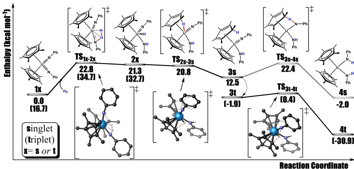
Fig. 5 B3PW91 enthalpy profile for the reaction of H 2 with (Me 5 C 5 ) 2 U(NPh) 2 .
