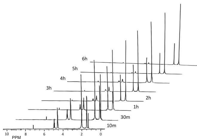
Fig. 1 Time evolution of the ^1H NMR spectrum for the reaction (Me_5C_5)_2Yb with buta-1,2-diene in C_6D_6 at 20^\circ C .
