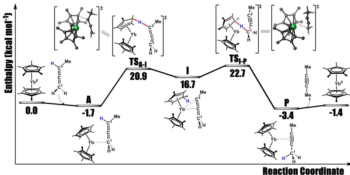
Fig. 2 B3PW91 enthalpy profile in kcal mol -1 for the 1,3-shift reaction mechanism in (Me 5 C 5 ) 2 Yb(buta-1,2-diene) to (Me 5 C 5 ) 2 Yb(MeCCMe).
